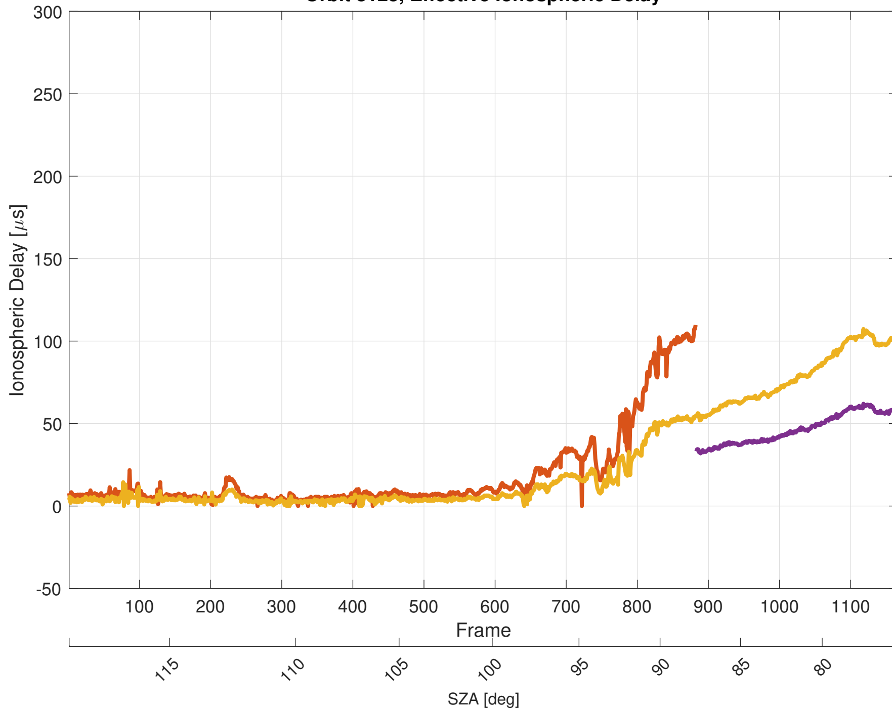
Orbit 8123, Effective Ionospheric Delay
