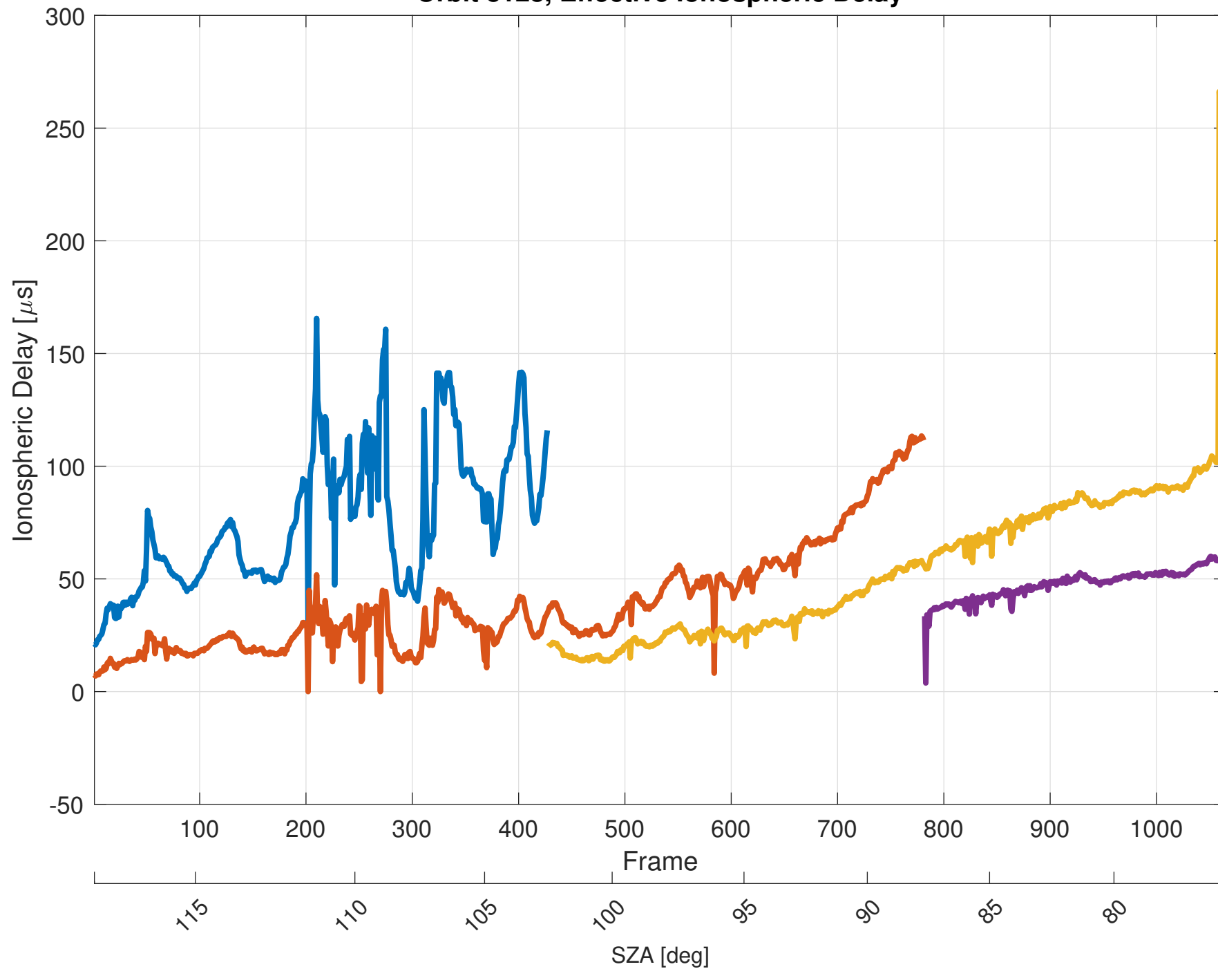
Orbit 8128, Effective Ionospheric Delay
