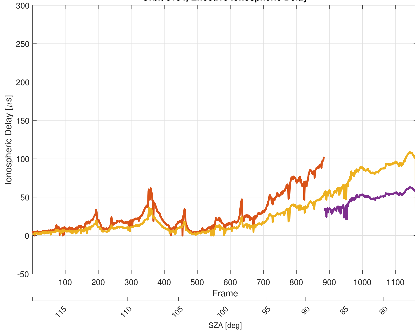
Orbit 8134, Effective Ionospheric Delay
