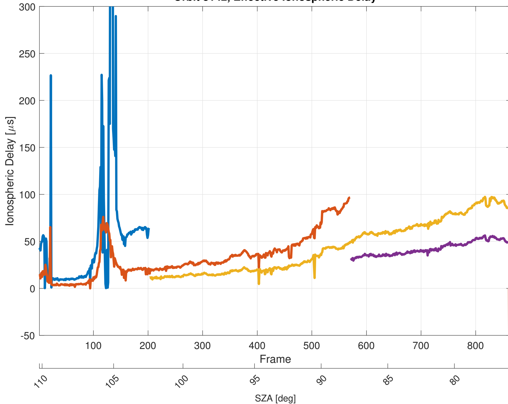
Orbit 8142, Effective Ionospheric Delay
