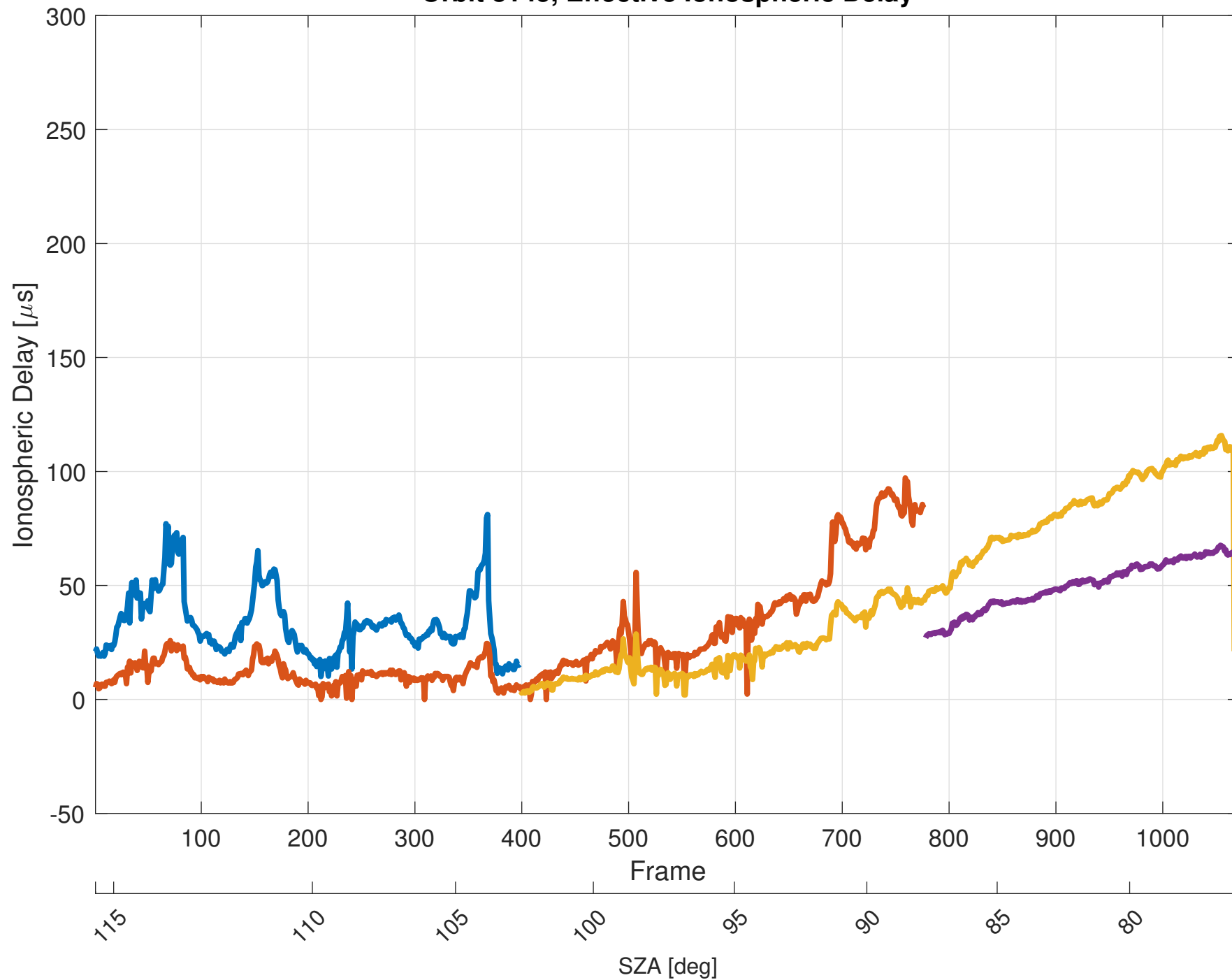
Orbit 8145, Effective Ionospheric Delay
