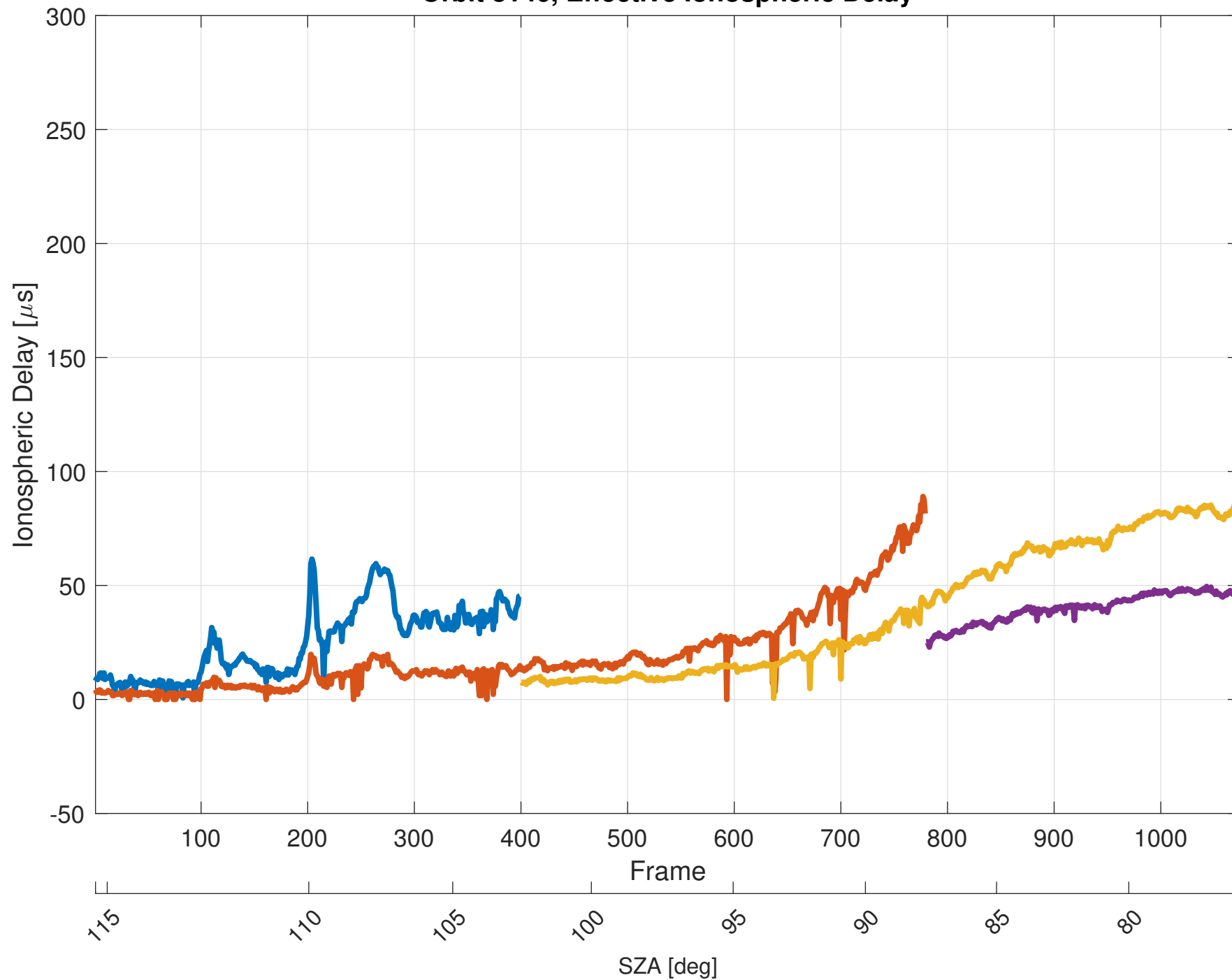
Orbit 8146, Effective Ionospheric Delay
