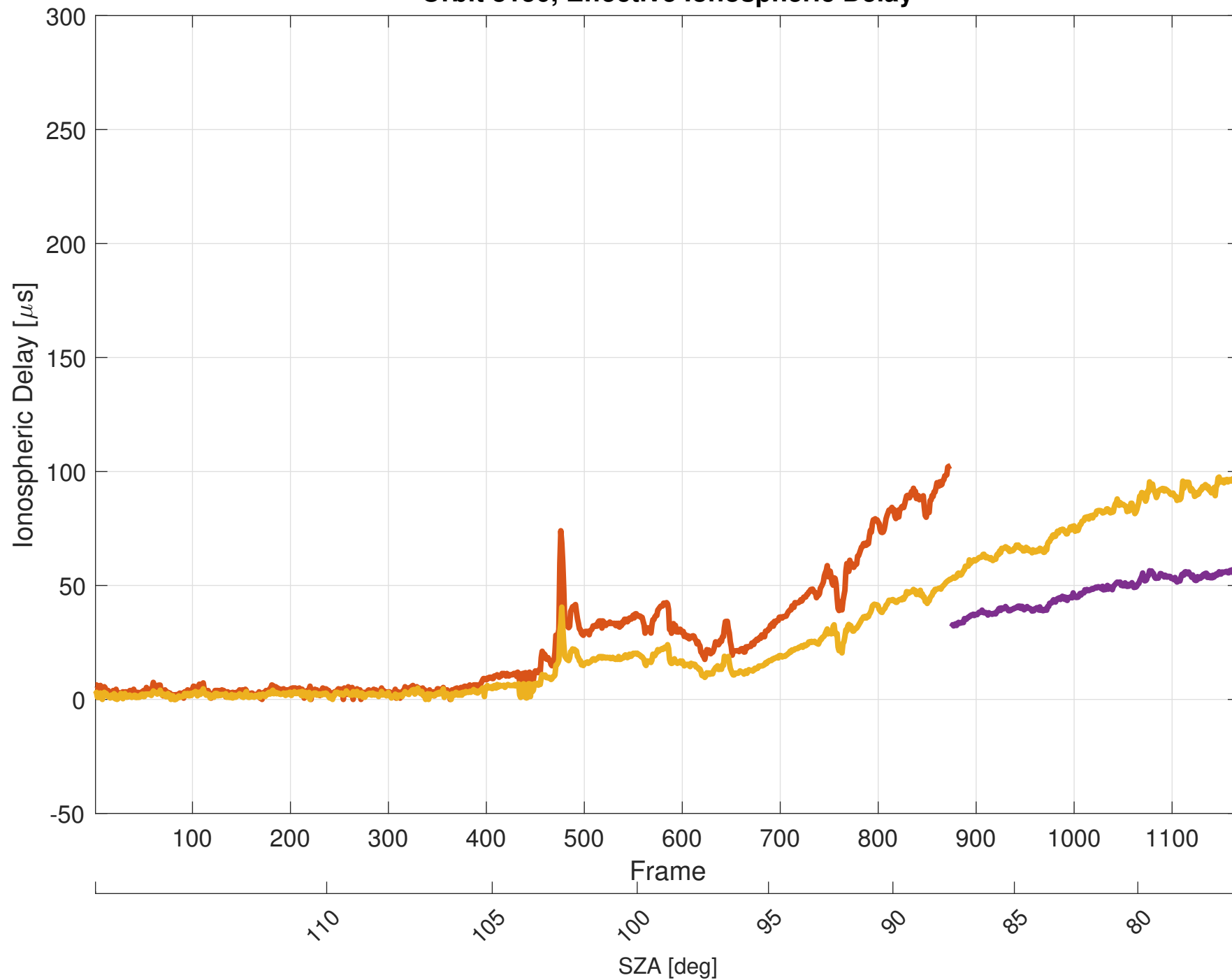
Orbit 8150, Effective Ionospheric Delay
