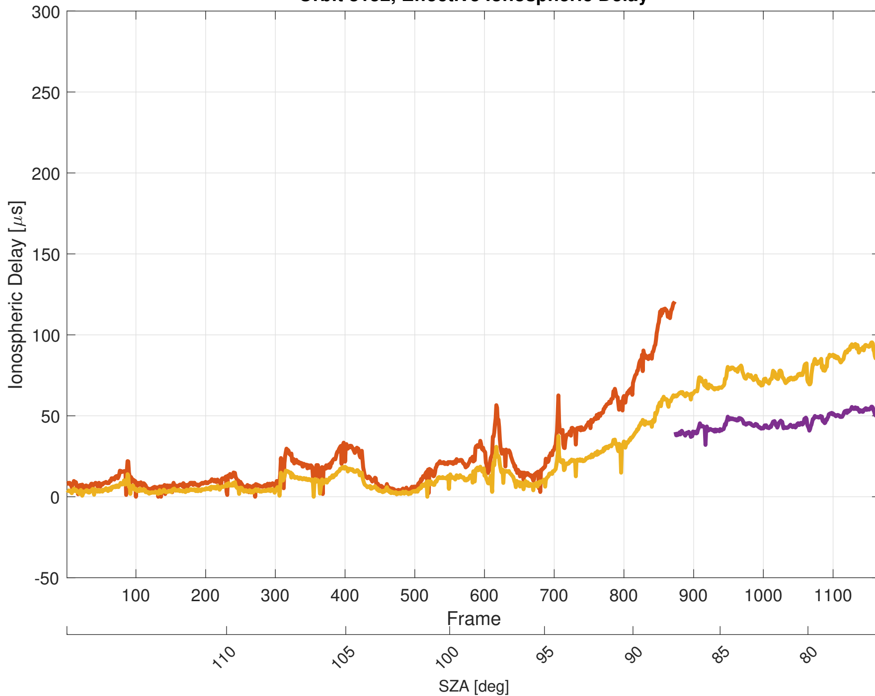
Orbit 8152, Effective Ionospheric Delay
