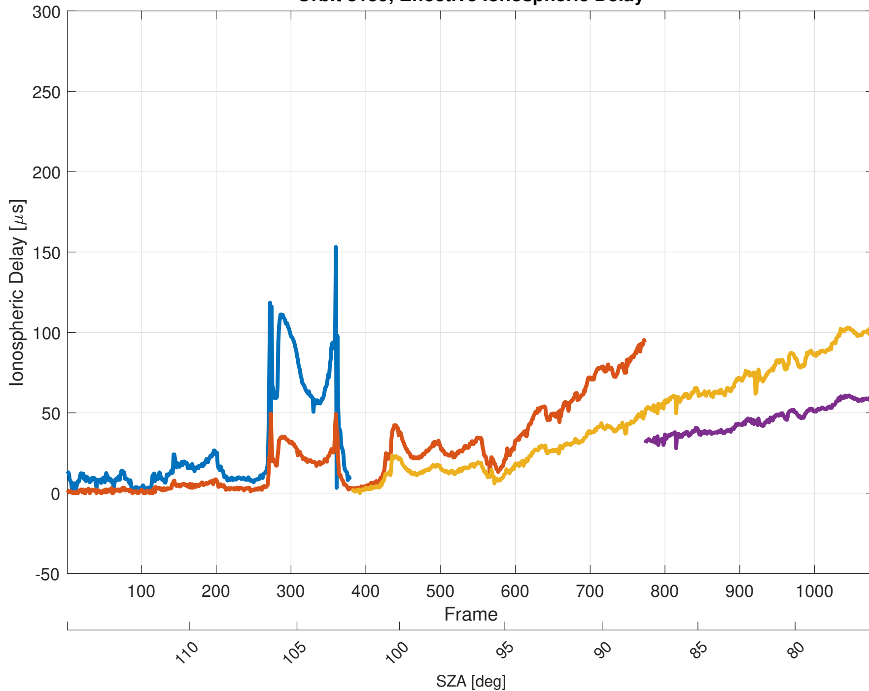
Orbit 8159, Effective Ionospheric Delay
