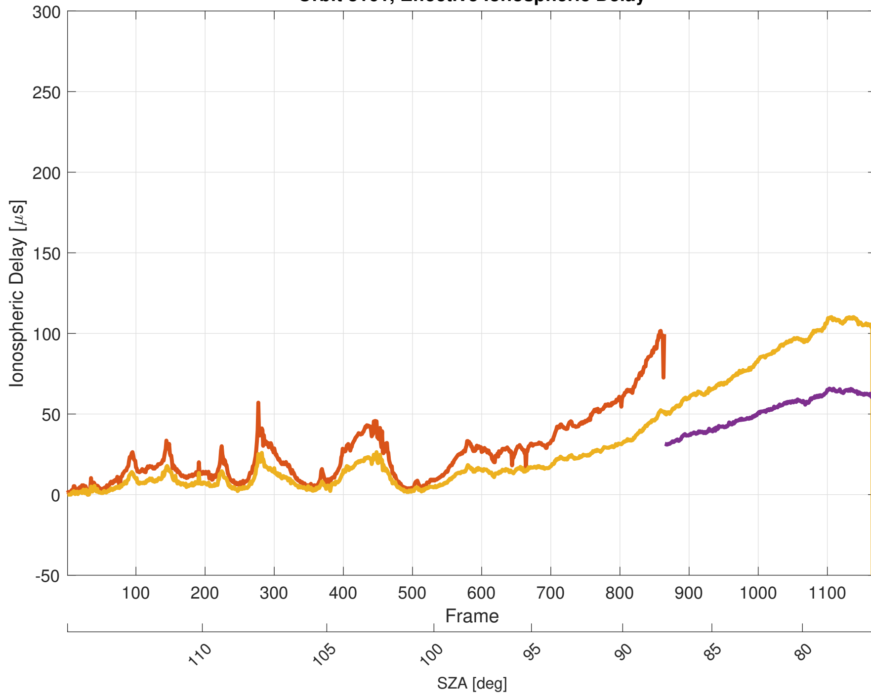
Orbit 8161, Effective Ionospheric Delay
