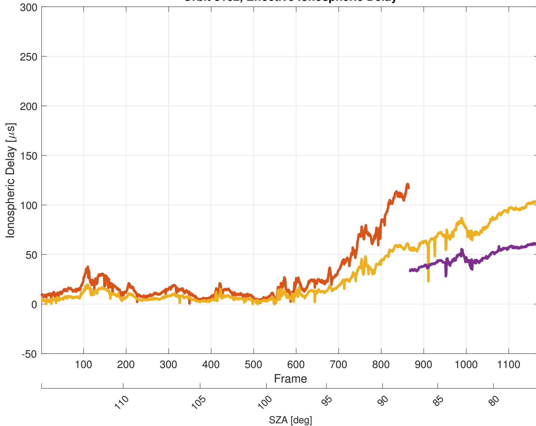
Orbit 8162, Effective Ionospheric Delay
