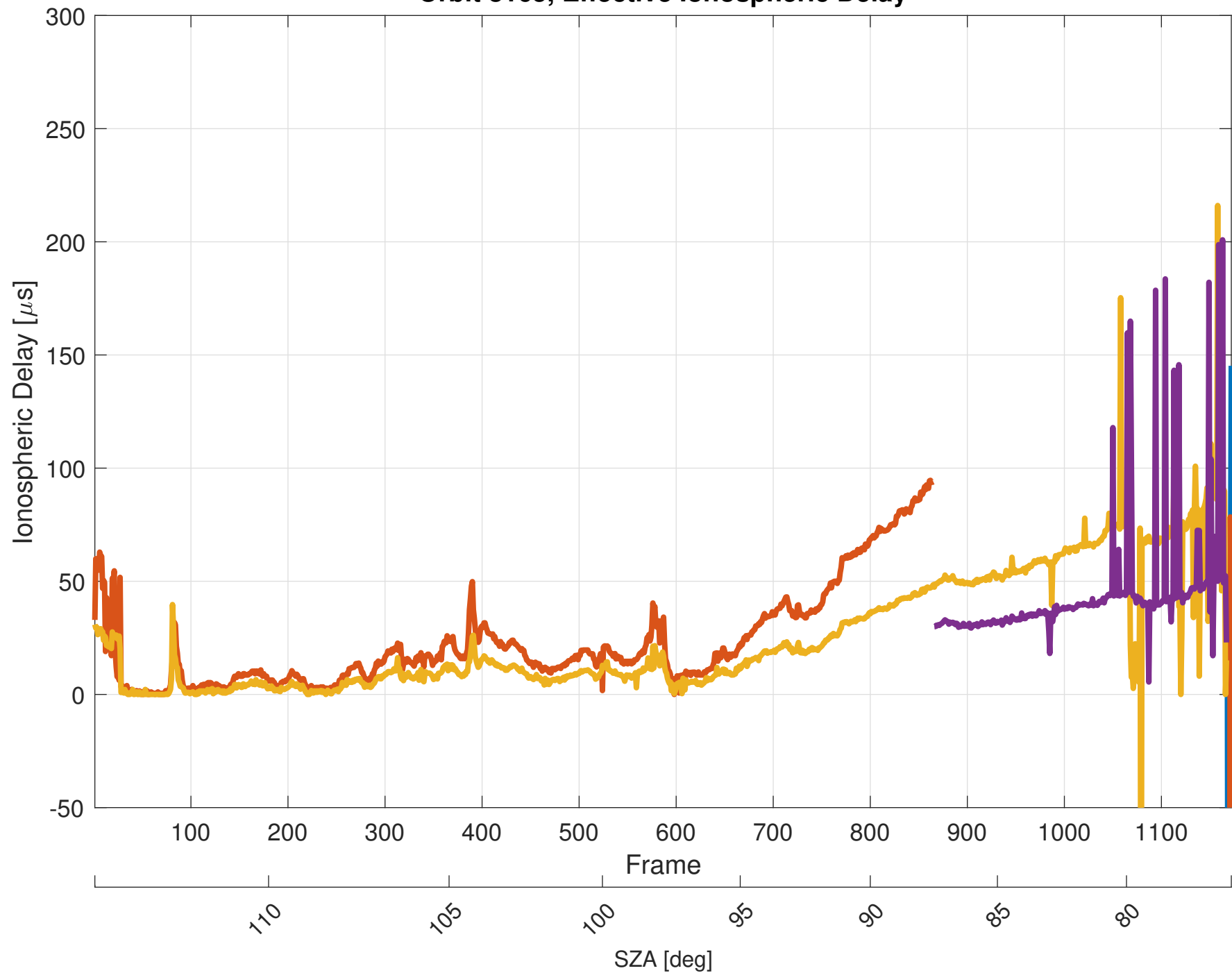
Orbit 8165, Effective Ionospheric Delay
