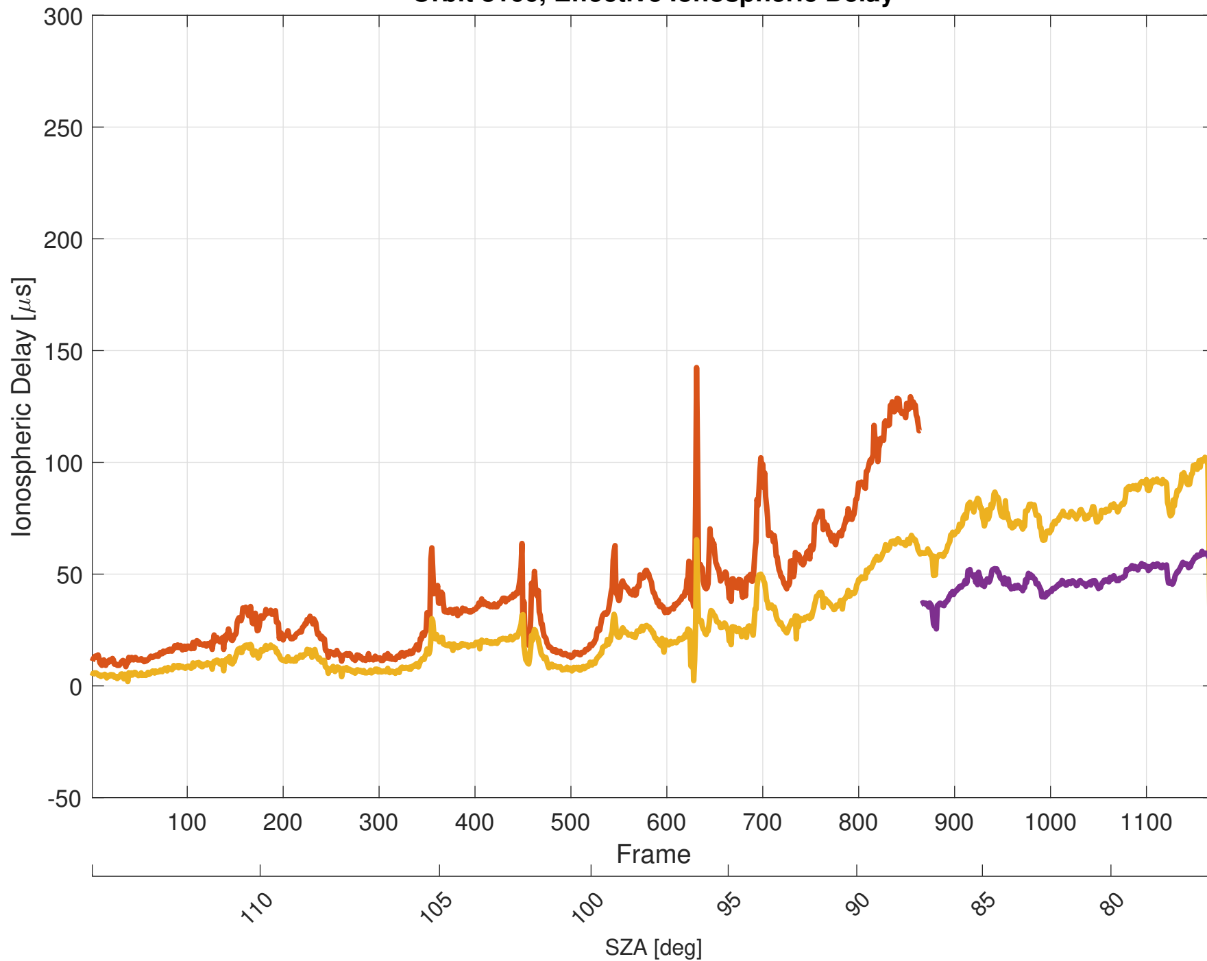
Orbit 8166, Effective Ionospheric Delay
