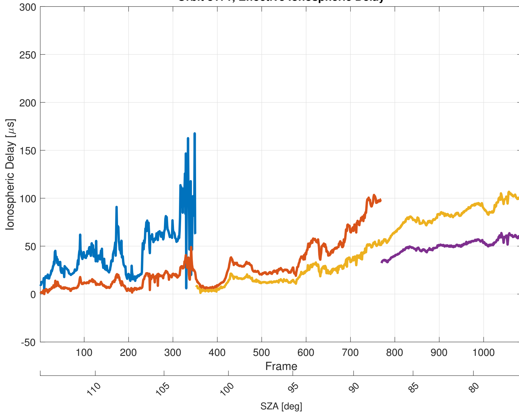
Orbit 8171, Effective Ionospheric Delay
