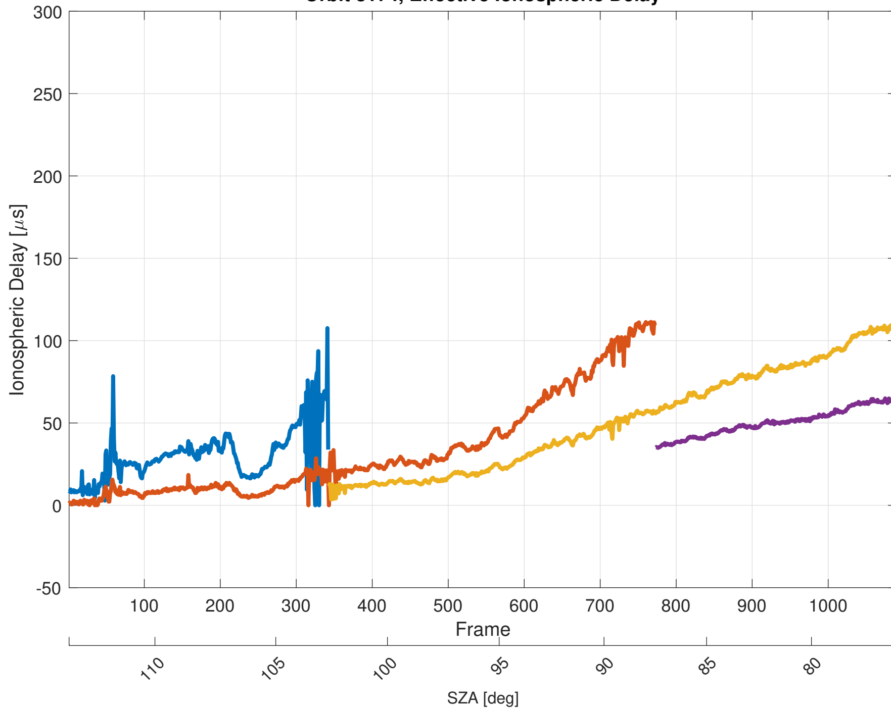
Orbit 8174, Effective Ionospheric Delay
