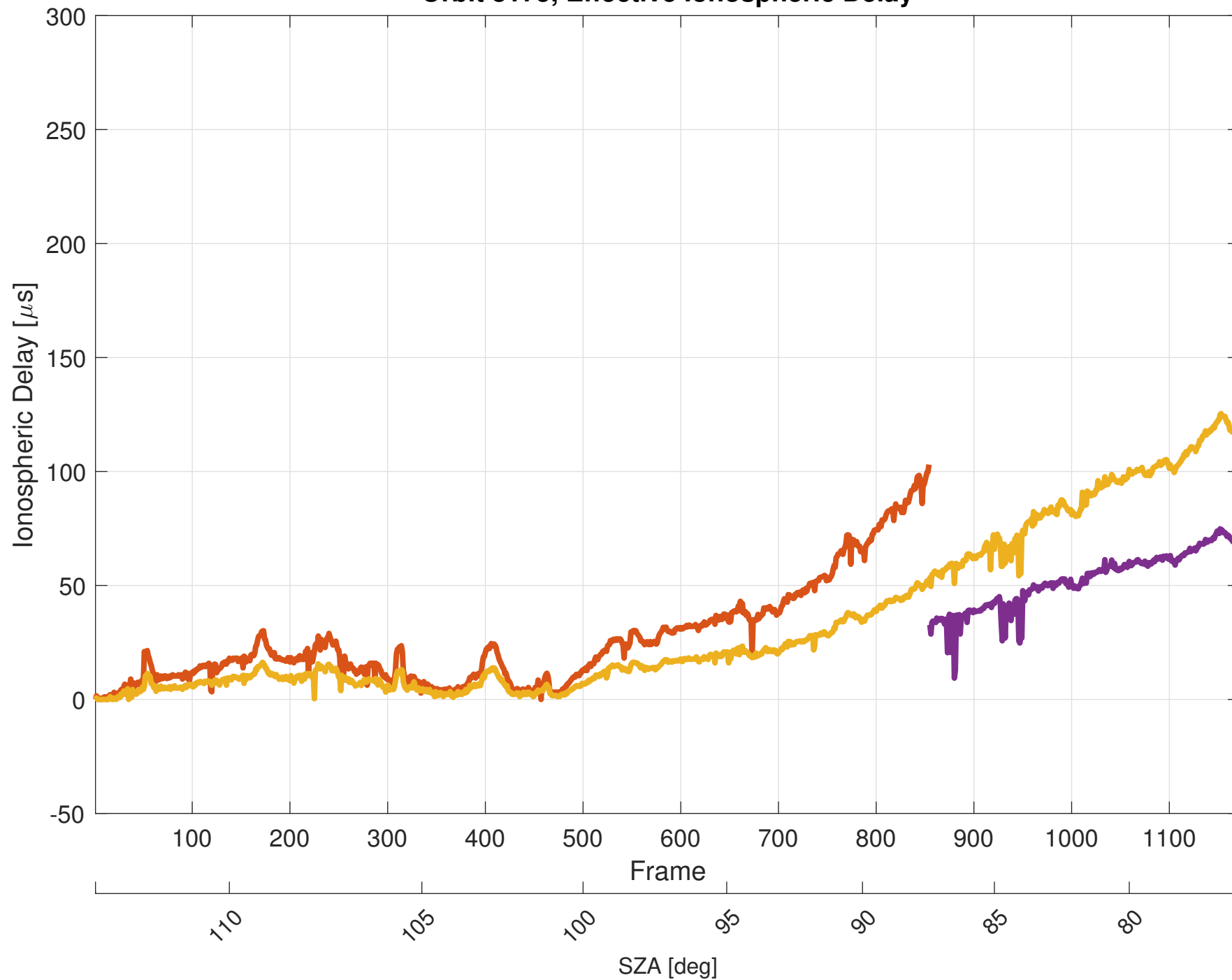
Orbit 8175, Effective Ionospheric Delay
