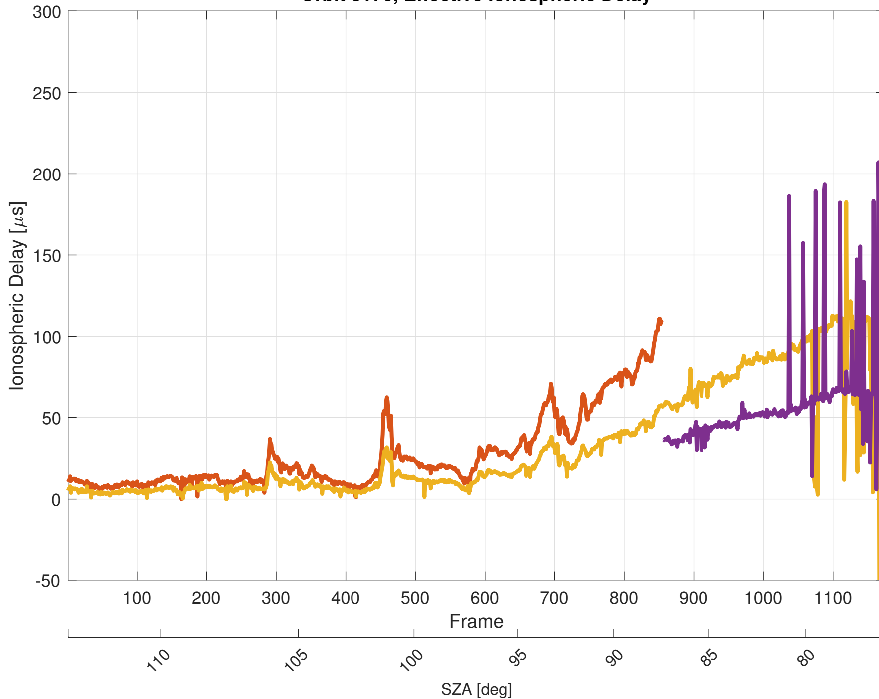
Orbit 8176, Effective Ionospheric Delay
