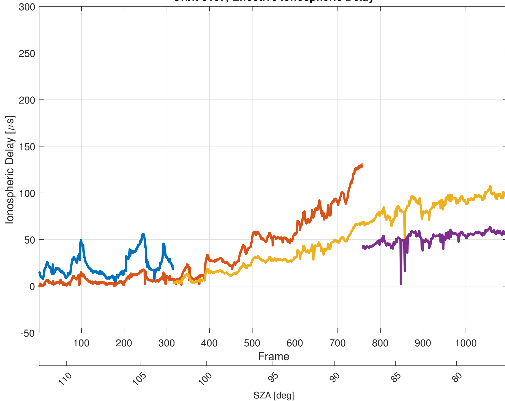
Orbit 8187, Effective Ionospheric Delay
