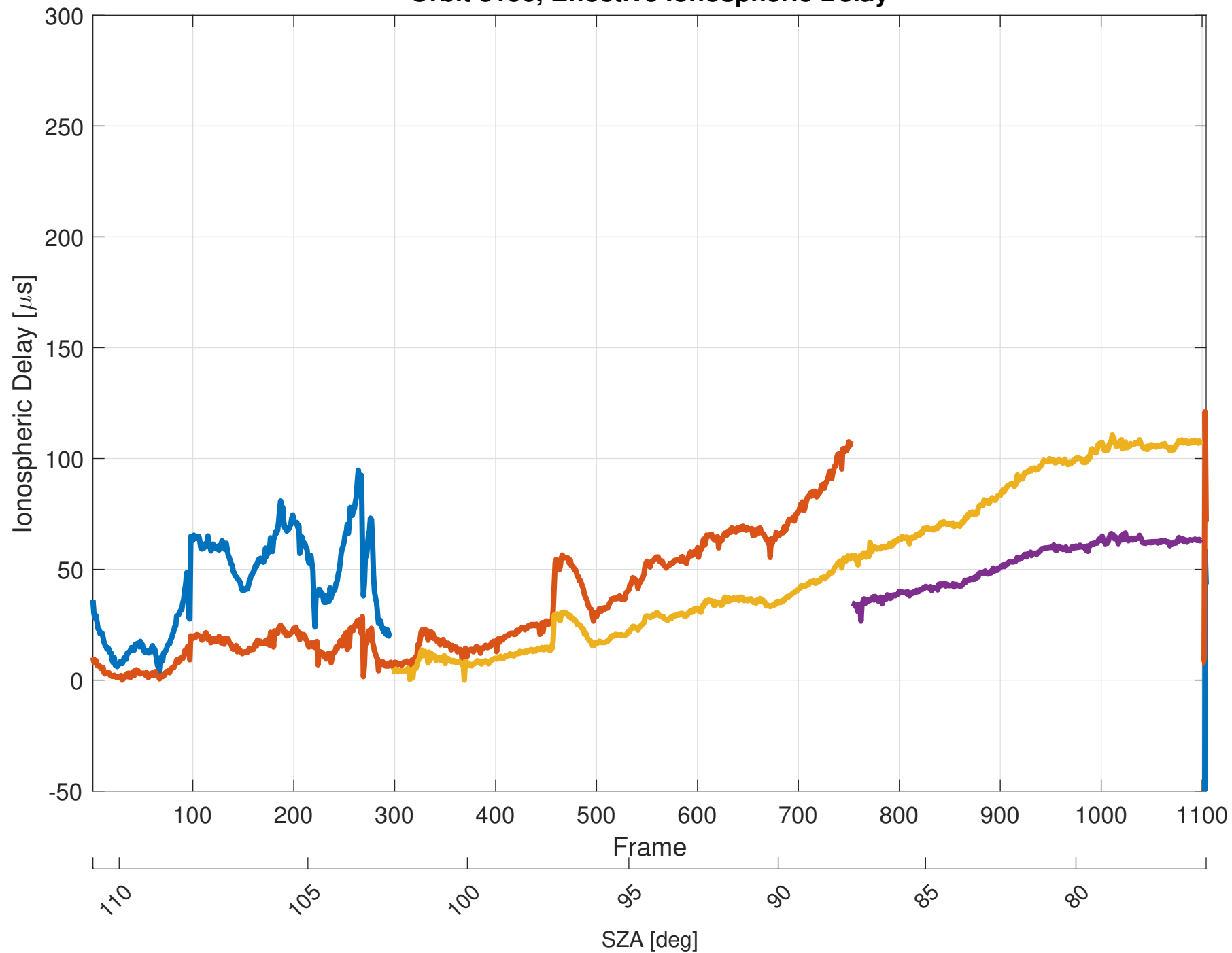
Orbit 8196, Effective Ionospheric Delay
