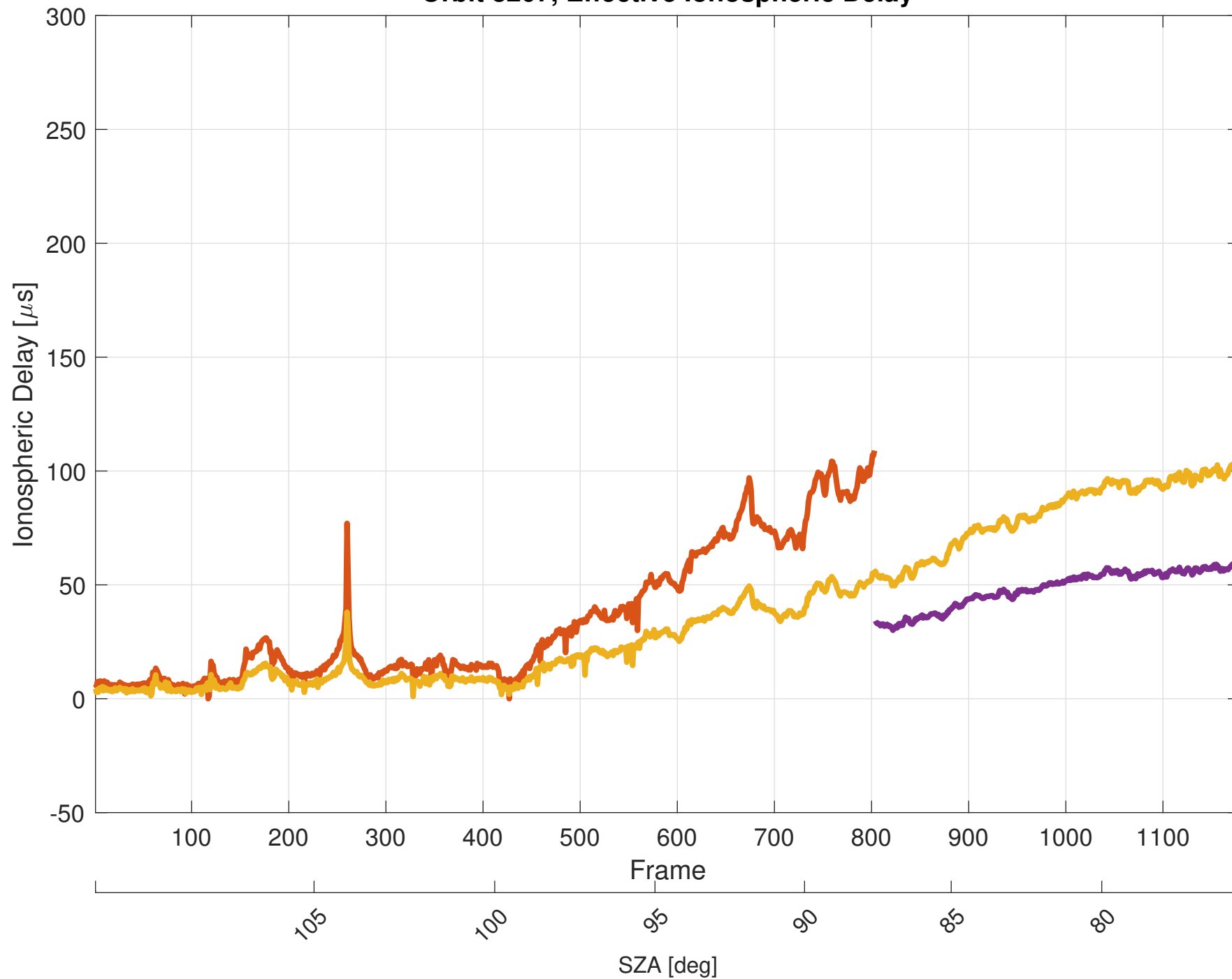
Orbit 8207, Effective Ionospheric Delay
