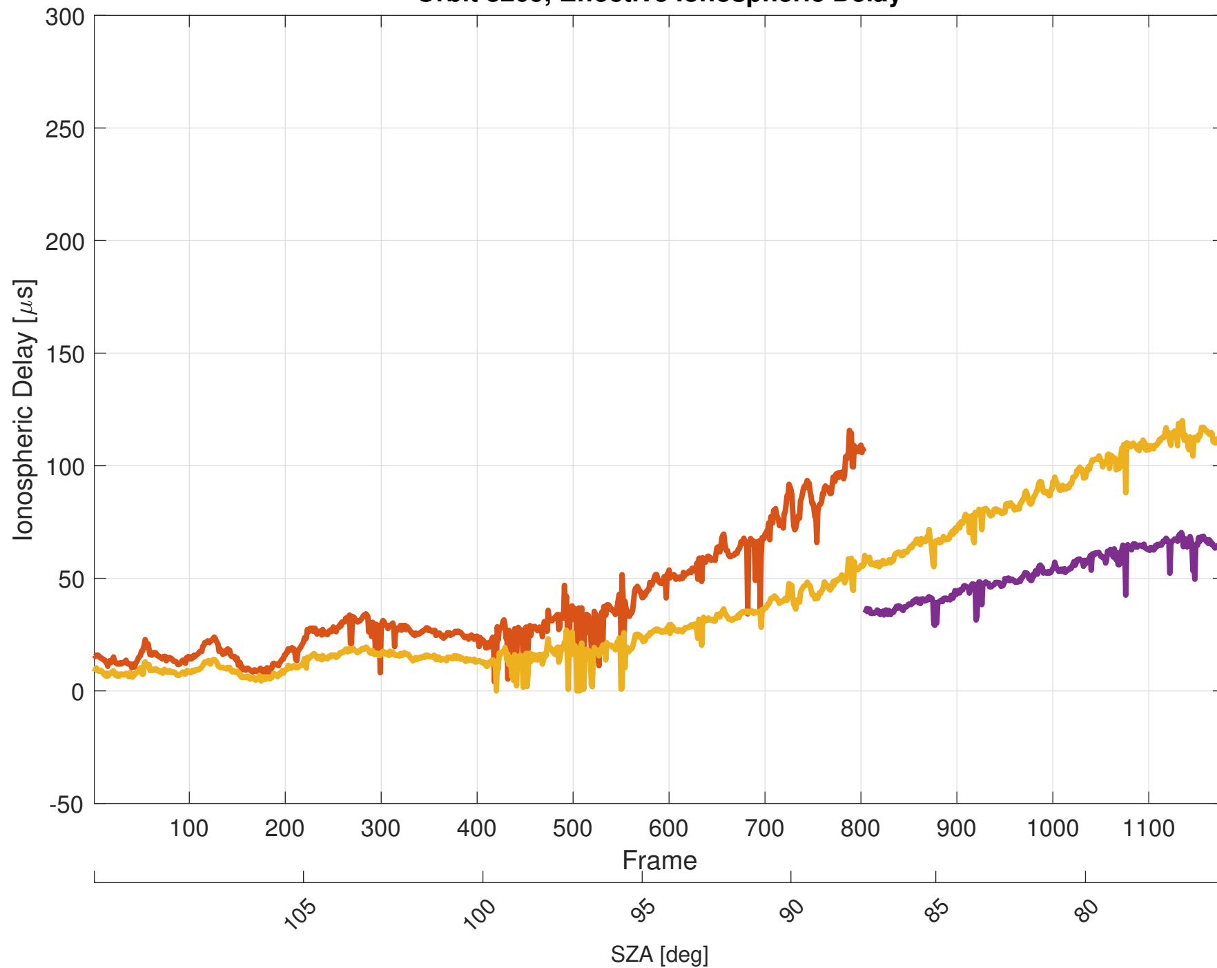
Orbit 8209, Effective Ionospheric Delay
