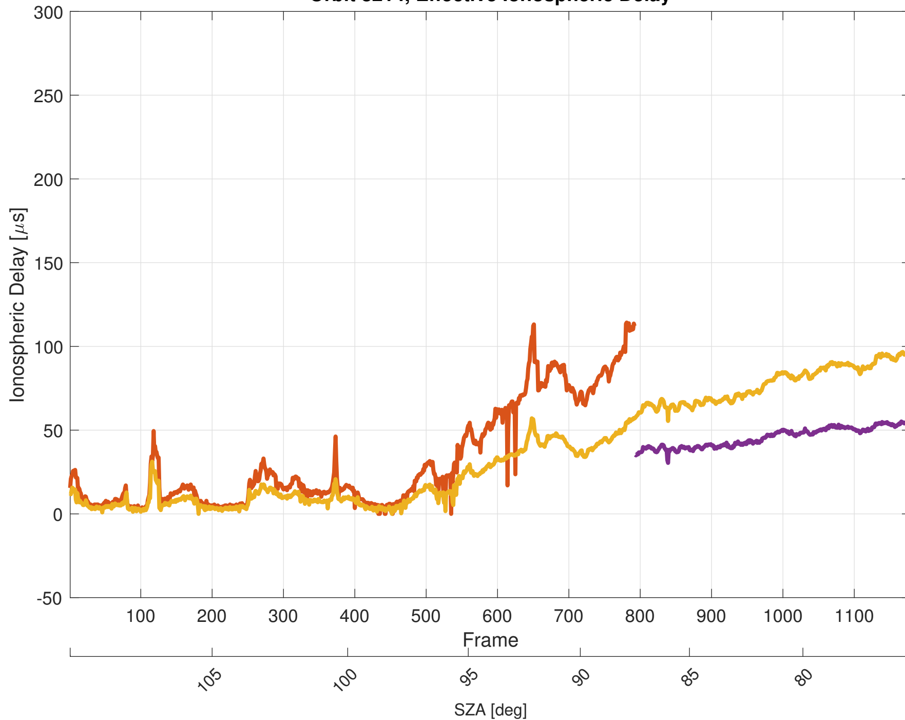
Orbit 8214, Effective Ionospheric Delay
