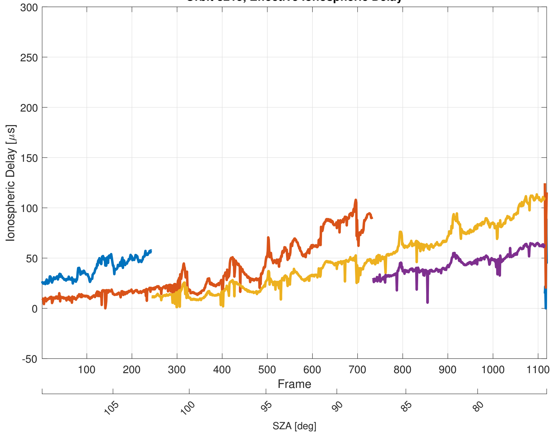
Orbit 8215, Effective Ionospheric Delay
