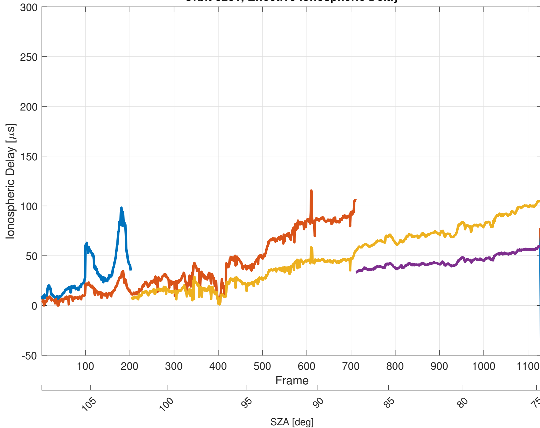
Orbit 8231, Effective Ionospheric Delay
