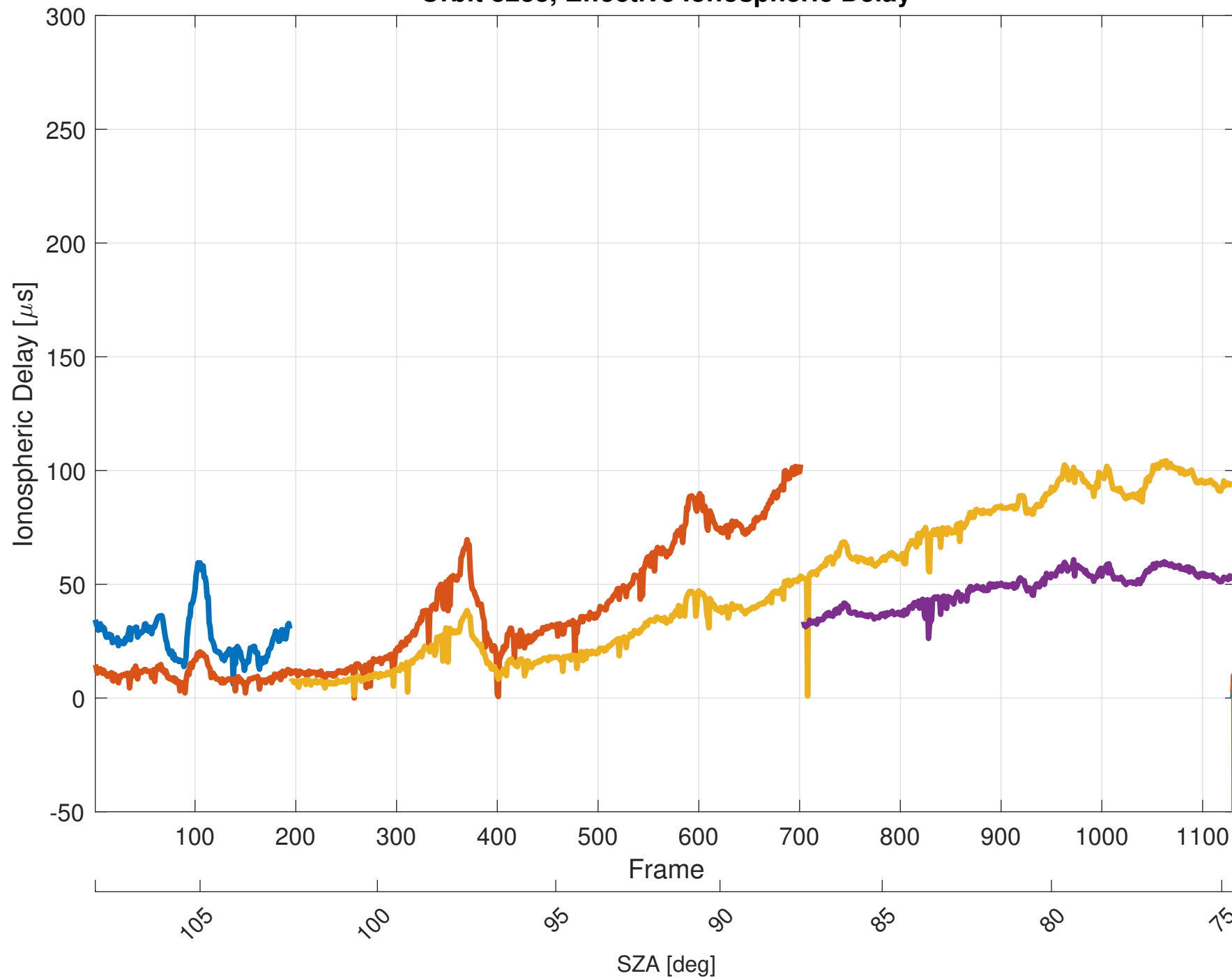
Orbit 8233, Effective Ionospheric Delay
