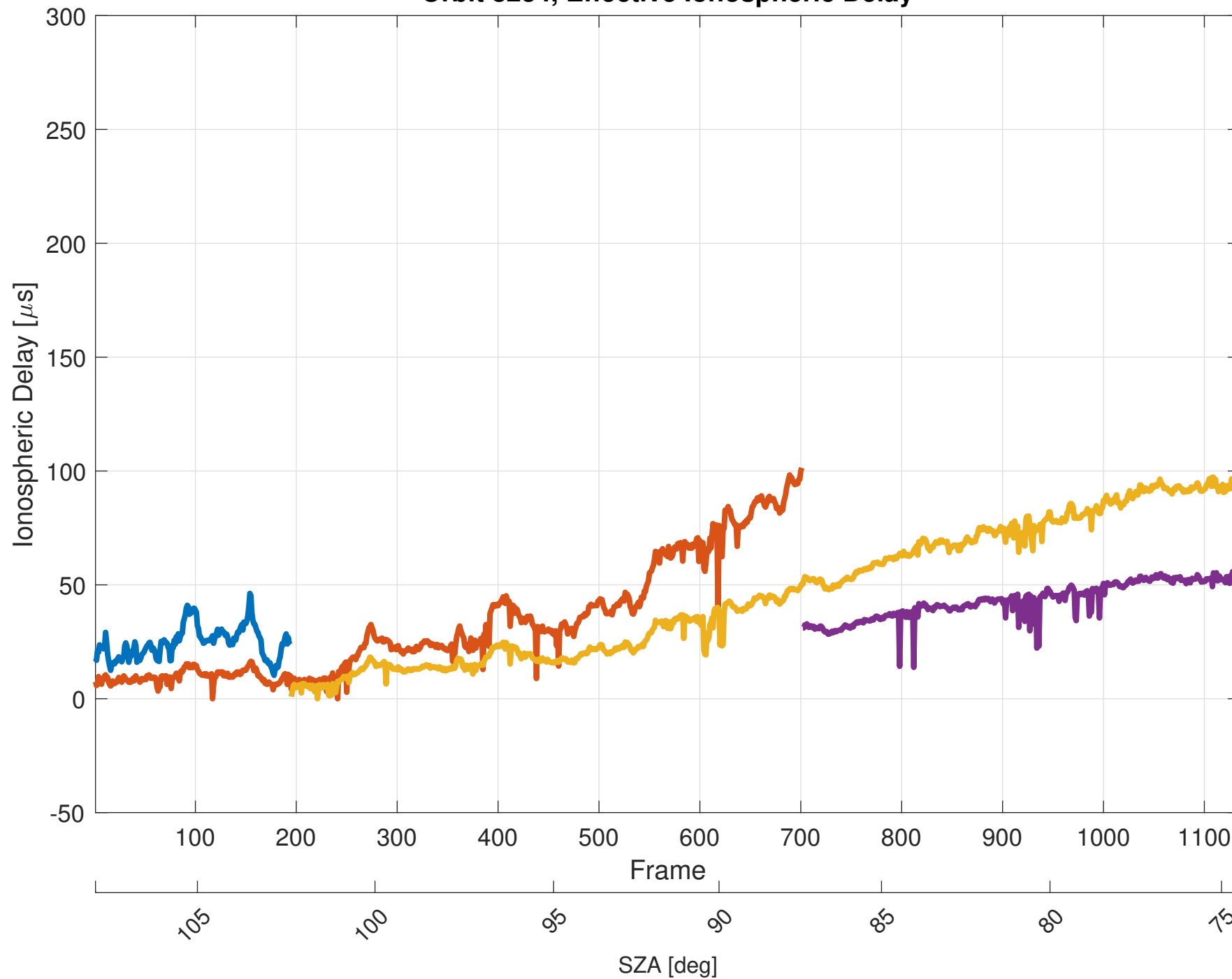
Orbit 8234, Effective Ionospheric Delay
