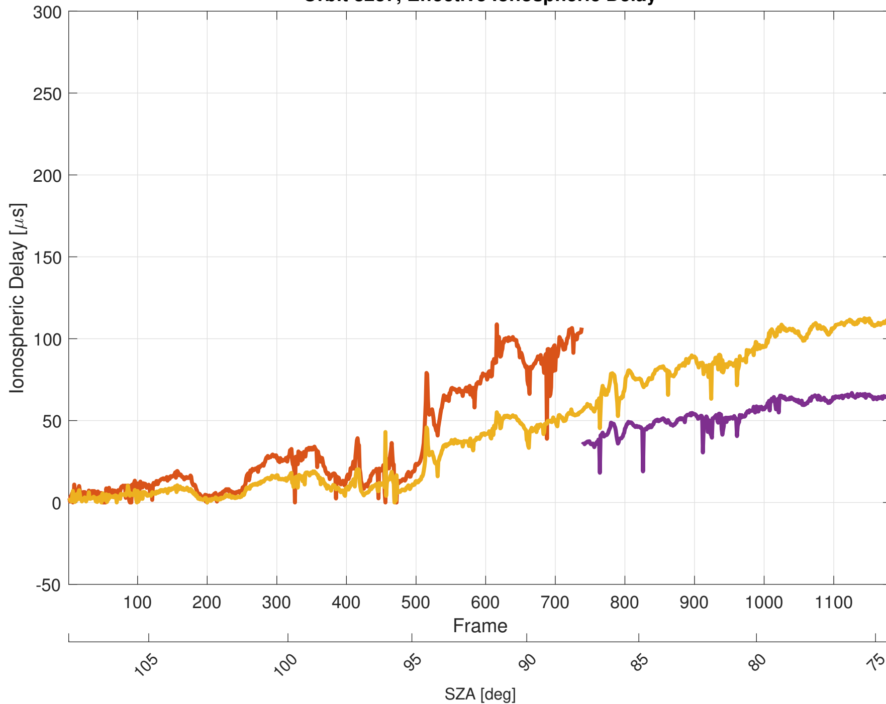
Orbit 8237, Effective Ionospheric Delay
