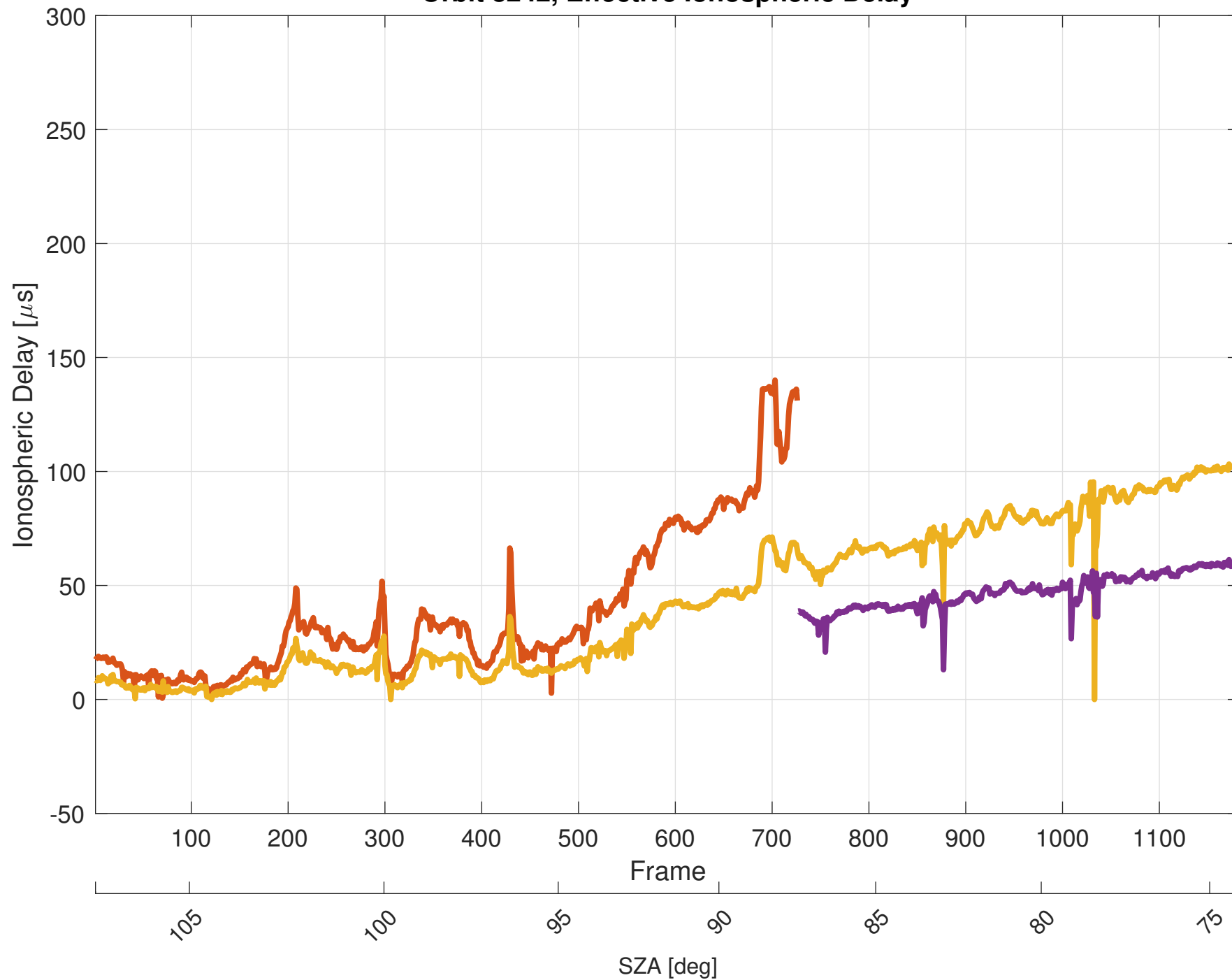
Orbit 8242, Effective Ionospheric Delay
