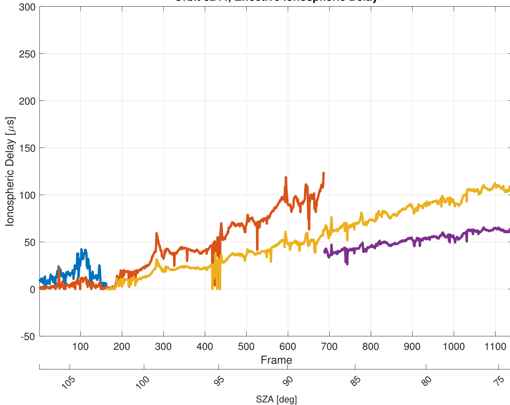
Orbit 8244, Effective Ionospheric Delay
