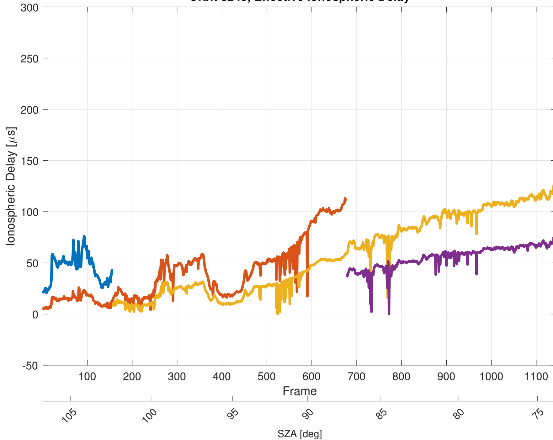
Orbit 8248, Effective Ionospheric Delay
