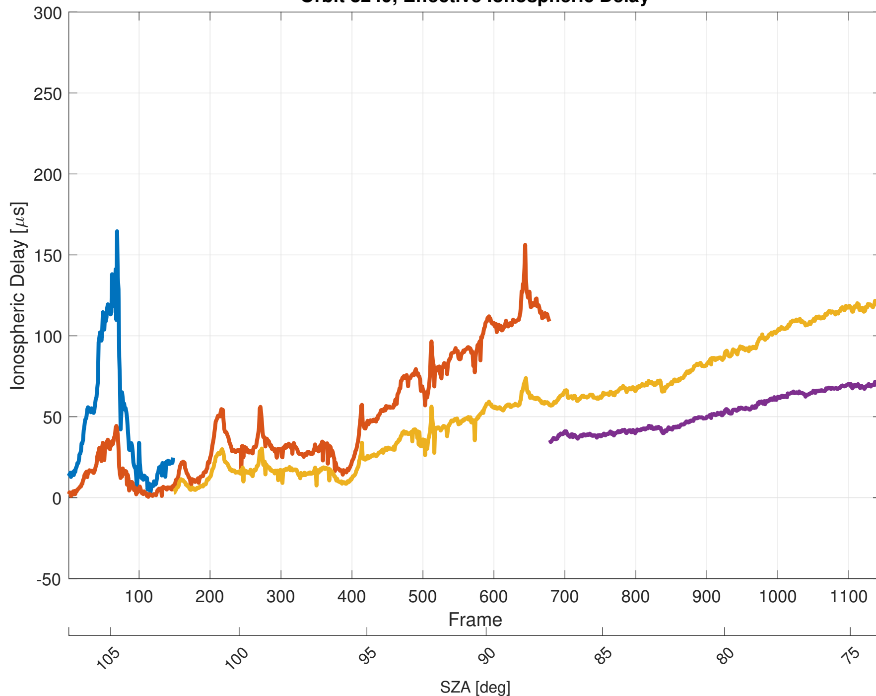
Orbit 8249, Effective Ionospheric Delay
