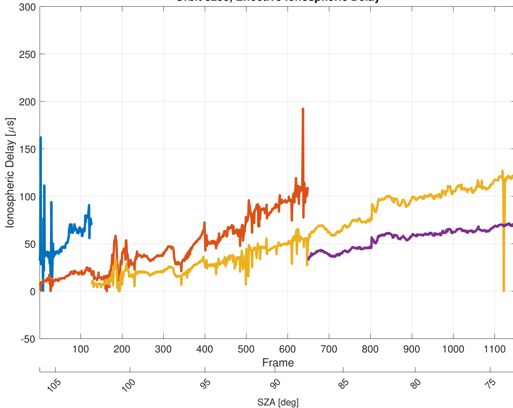
Orbit 8258, Effective Ionospheric Delay
