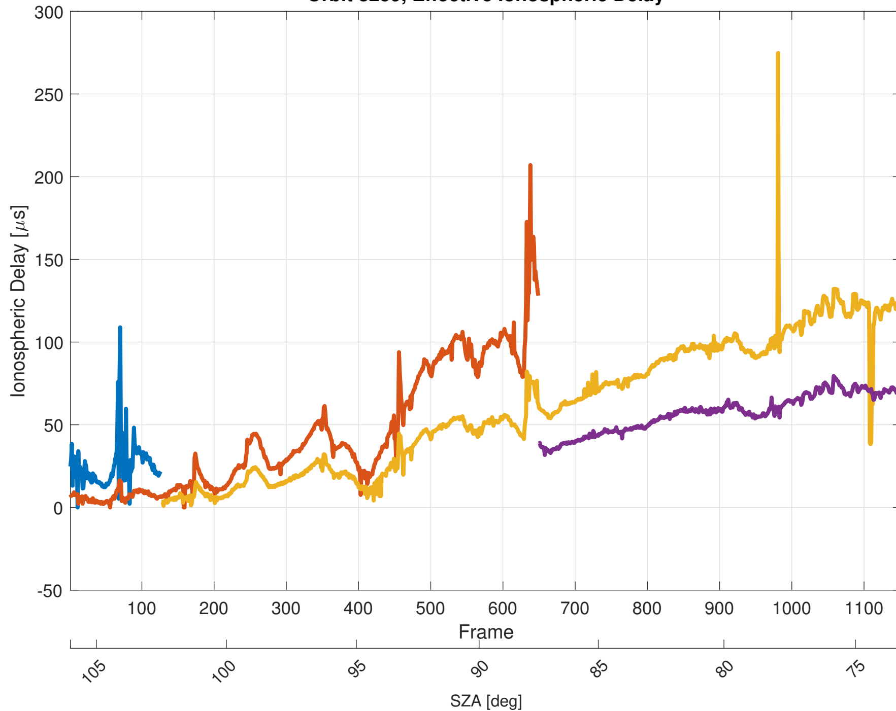
Orbit 8259, Effective Ionospheric Delay
