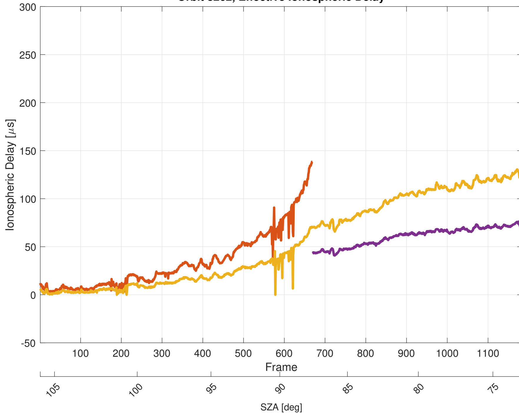
Orbit 8262, Effective Ionospheric Delay
