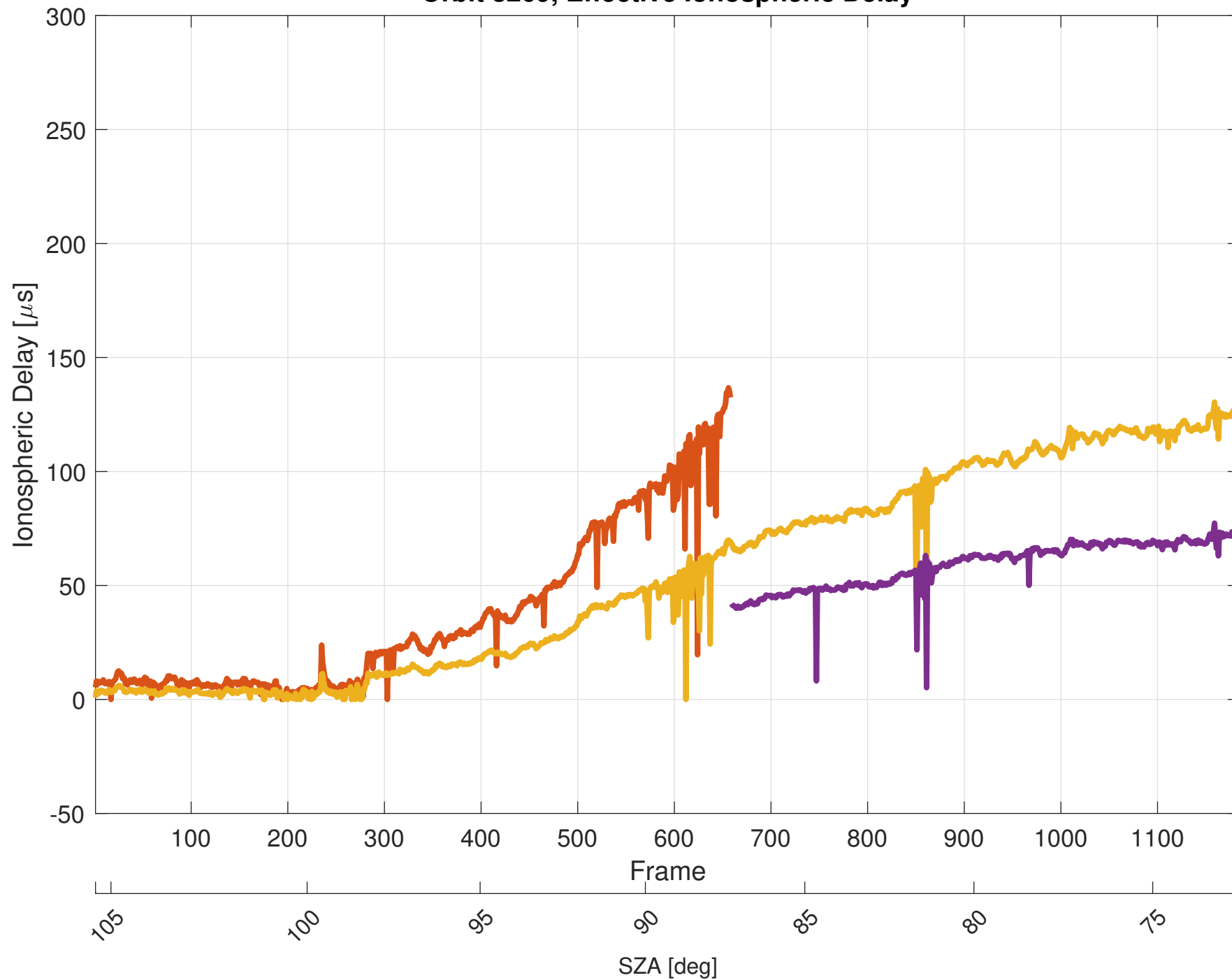
Orbit 8269, Effective Ionospheric Delay
