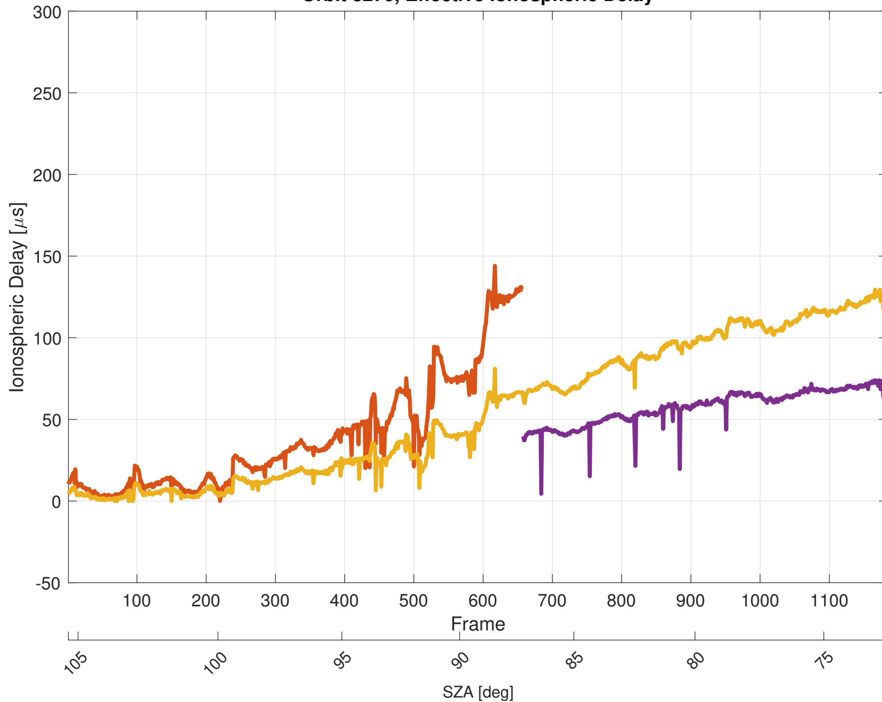
Orbit 8270, Effective Ionospheric Delay
