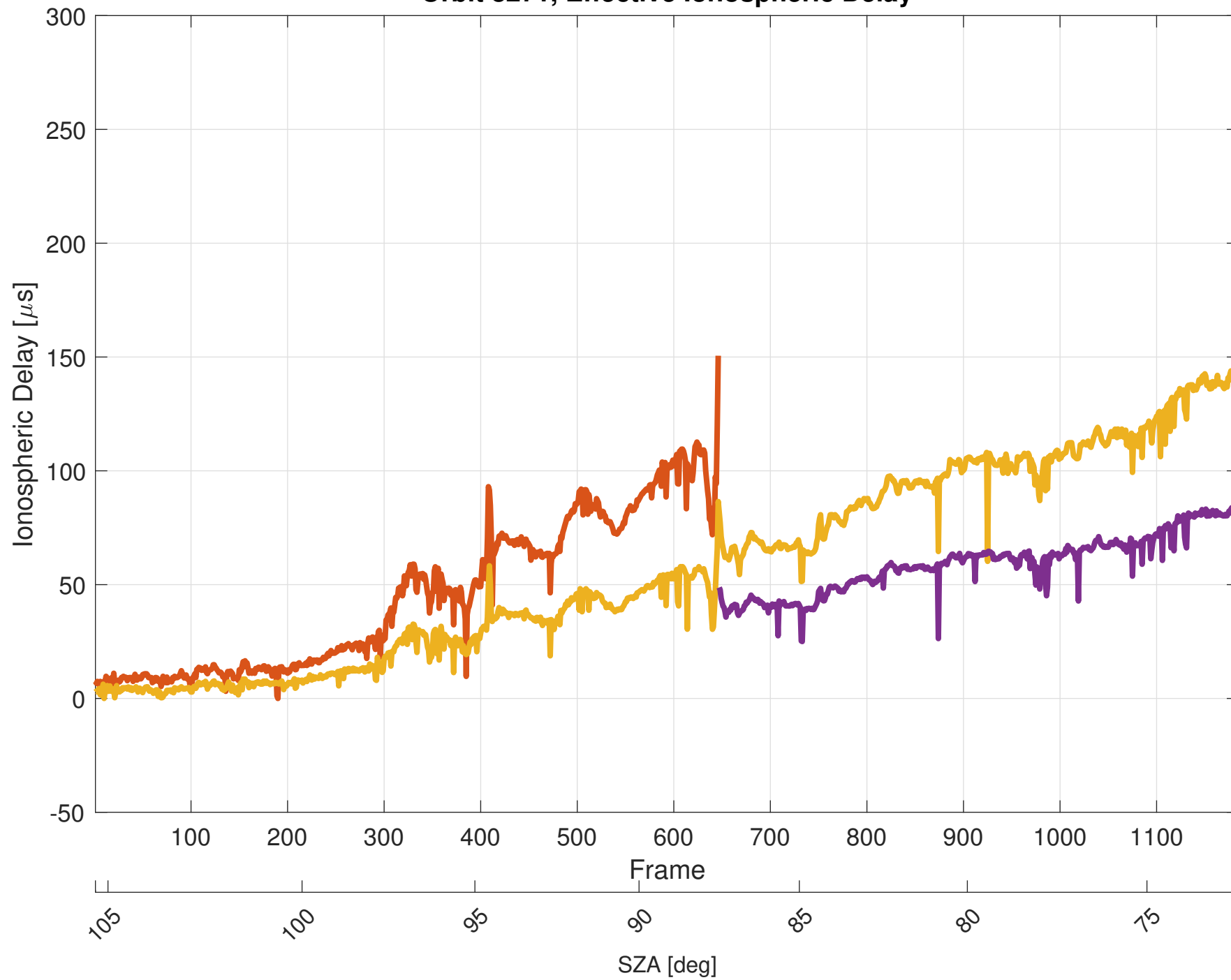
Orbit 8271, Effective Ionospheric Delay
