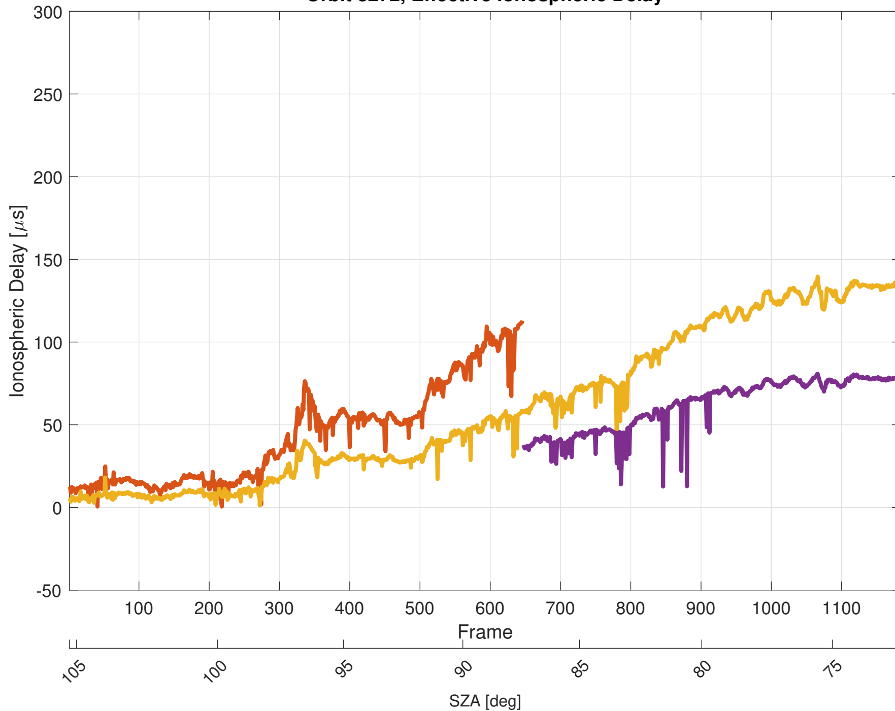
Orbit 8272, Effective Ionospheric Delay
