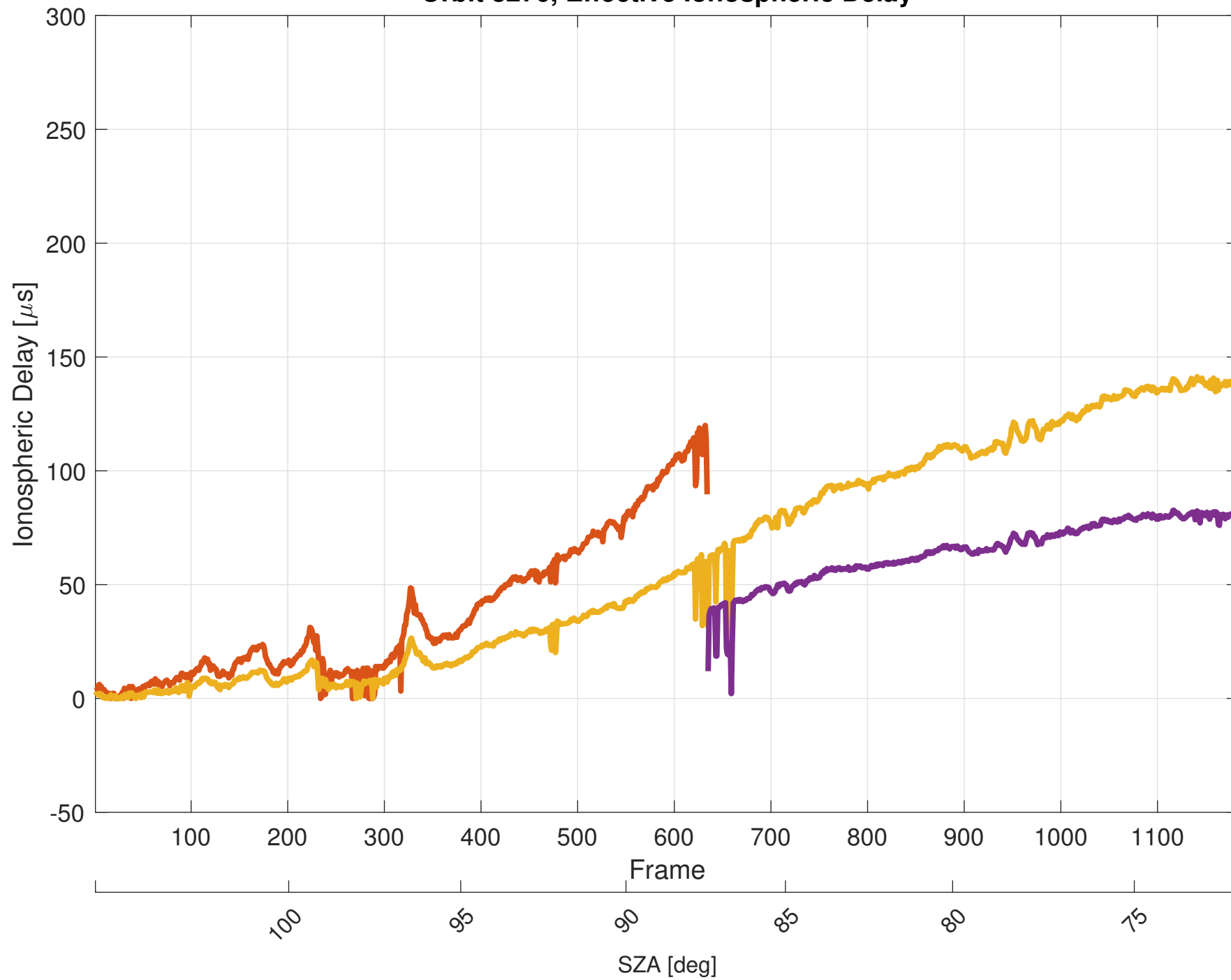
Orbit 8276, Effective Ionospheric Delay
