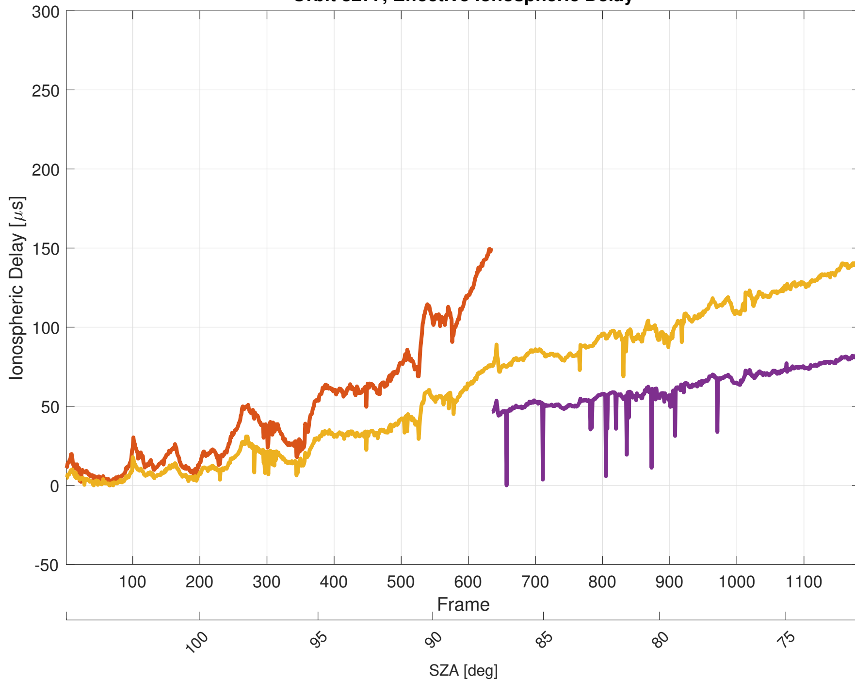
Orbit 8277, Effective Ionospheric Delay
