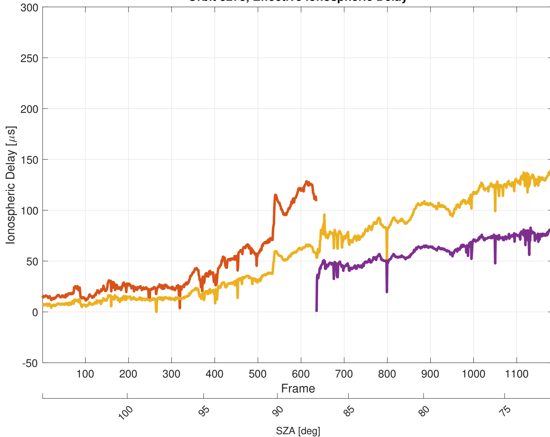
Orbit 8278, Effective Ionospheric Delay
