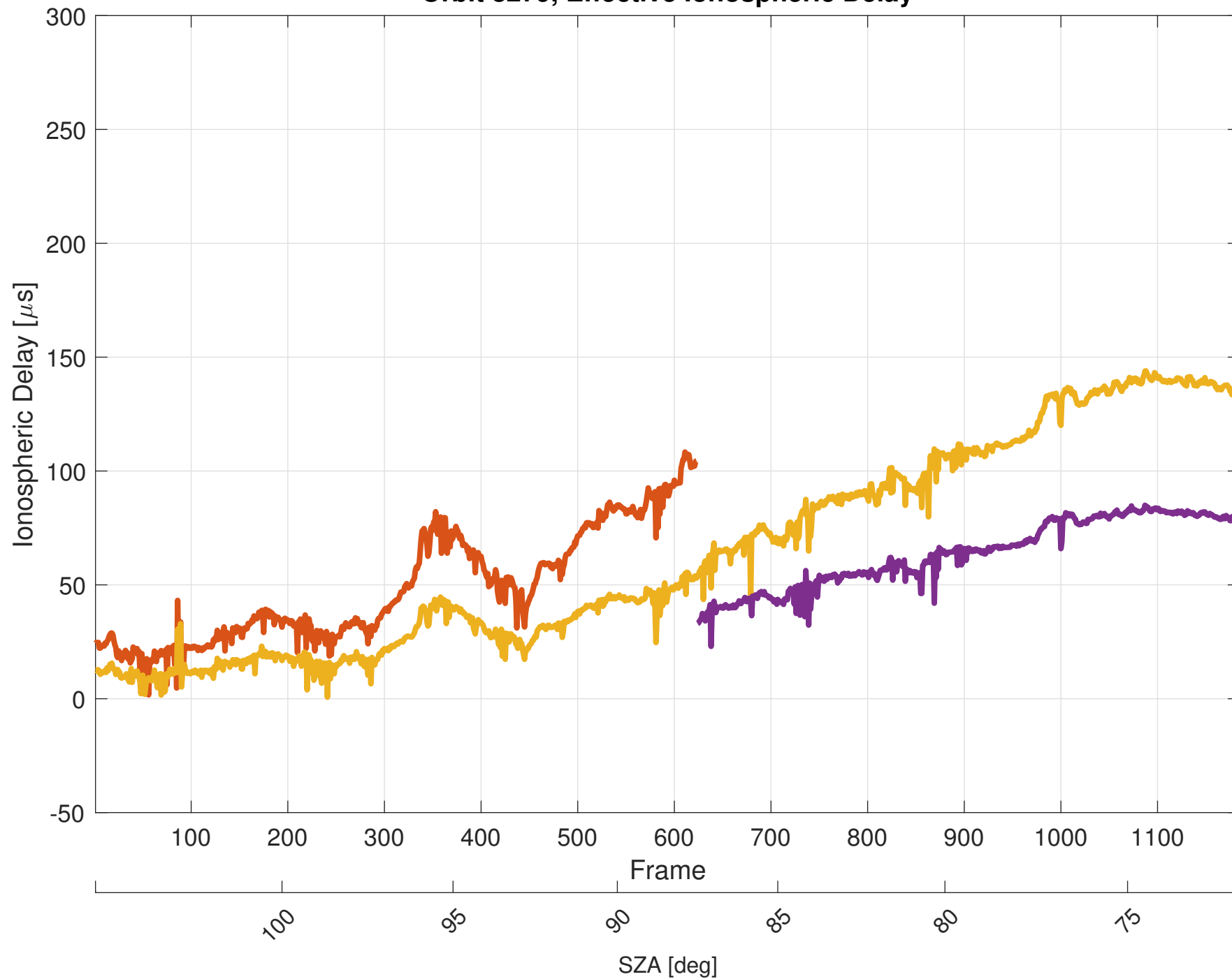
Orbit 8279, Effective Ionospheric Delay
