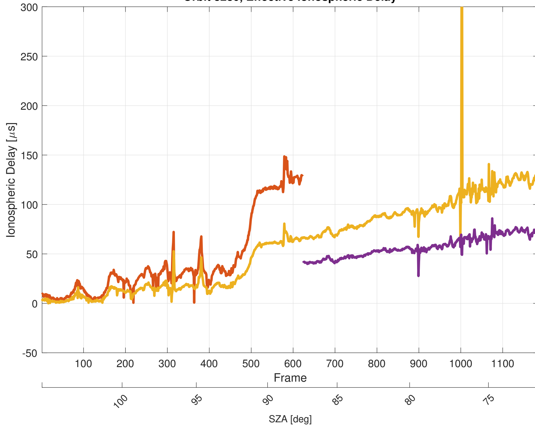
Orbit 8280, Effective Ionospheric Delay
