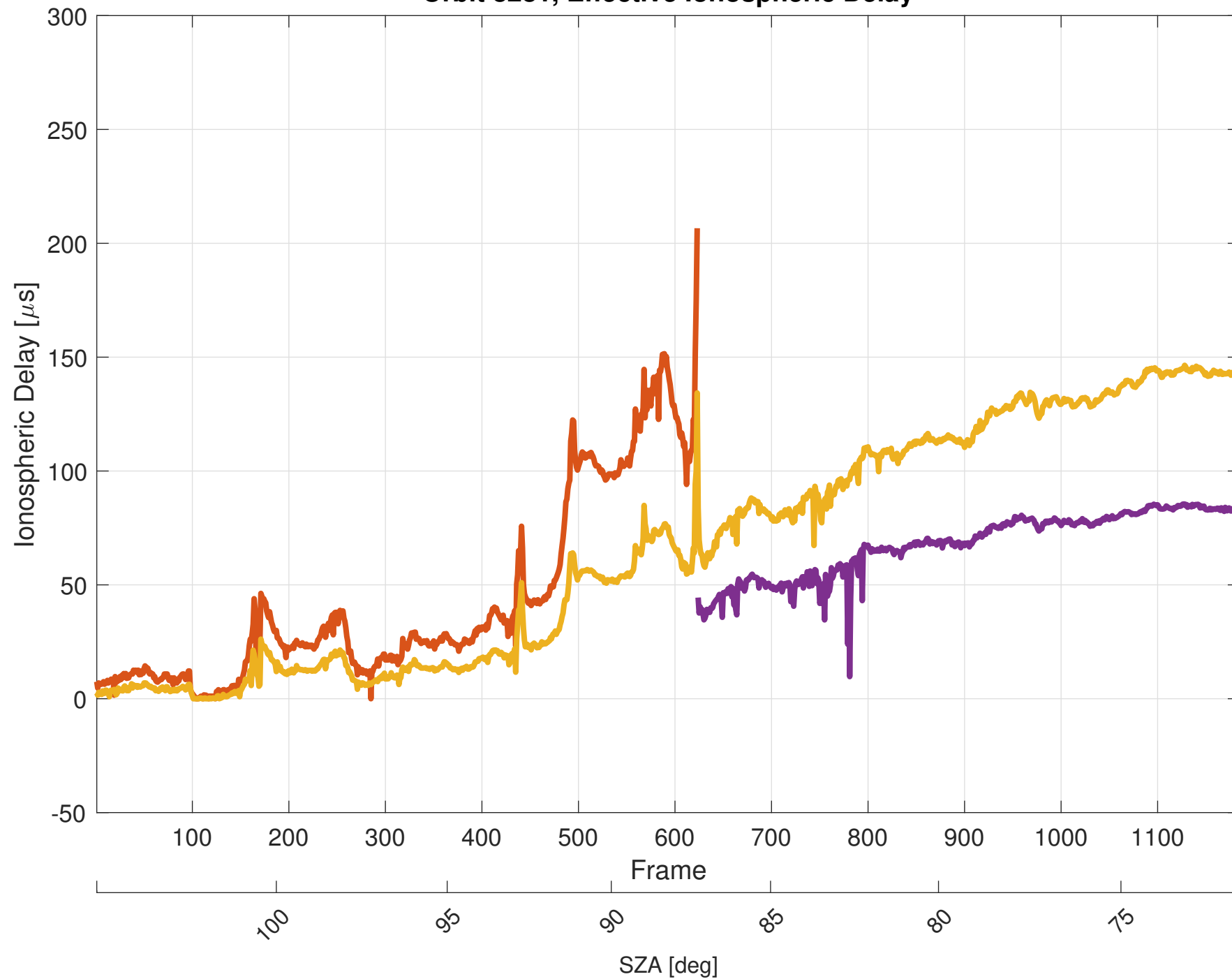
Orbit 8281, Effective Ionospheric Delay
