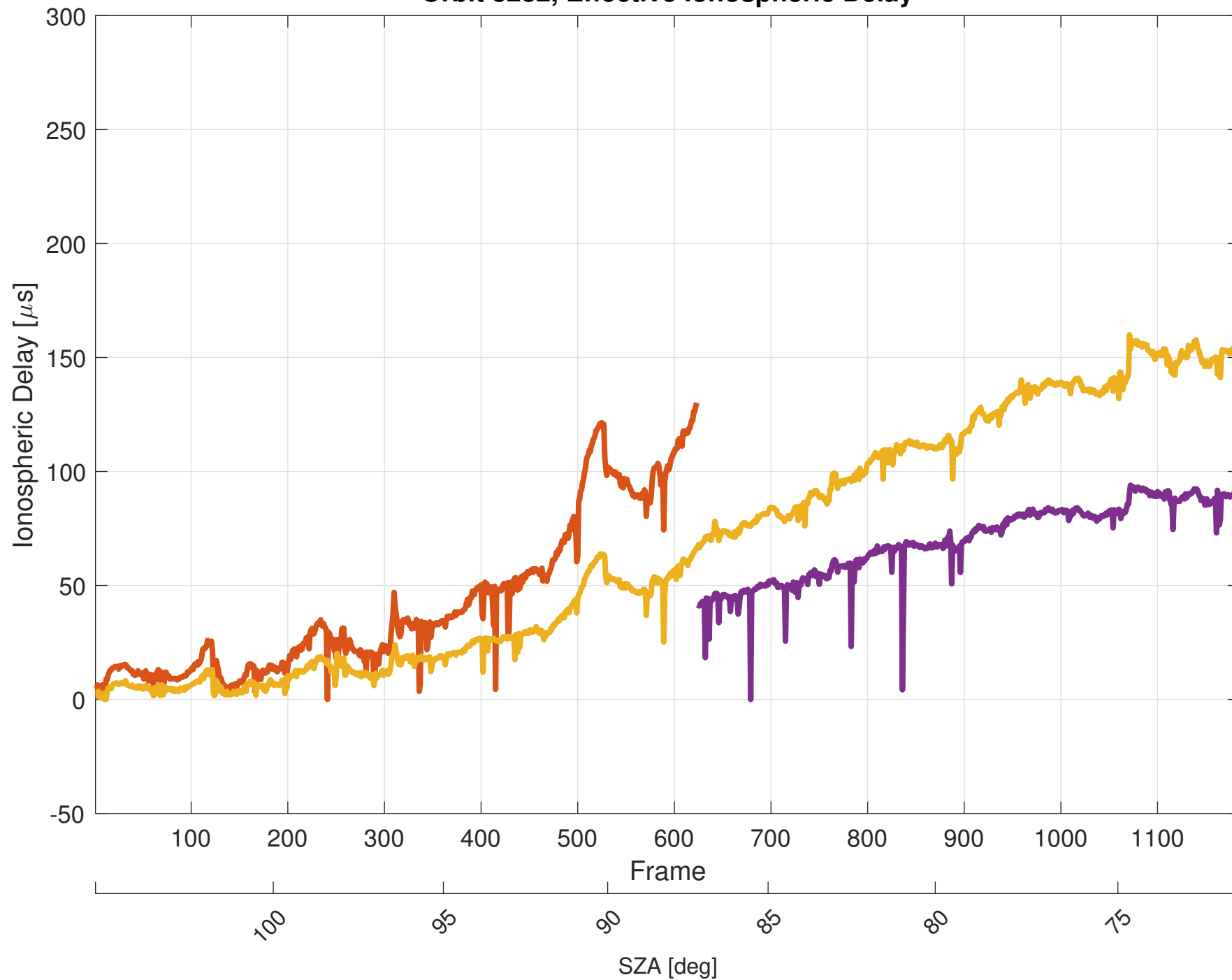
Orbit 8282, Effective Ionospheric Delay
