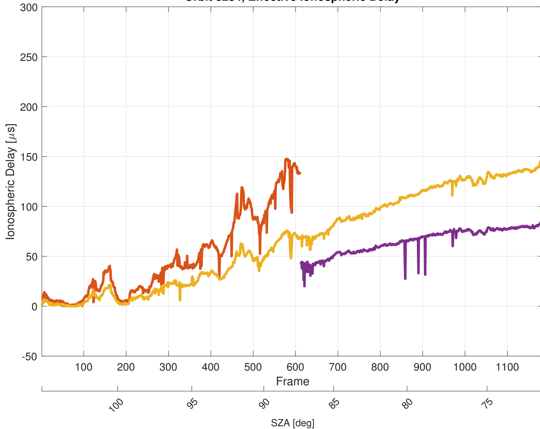
Orbit 8284, Effective Ionospheric Delay
