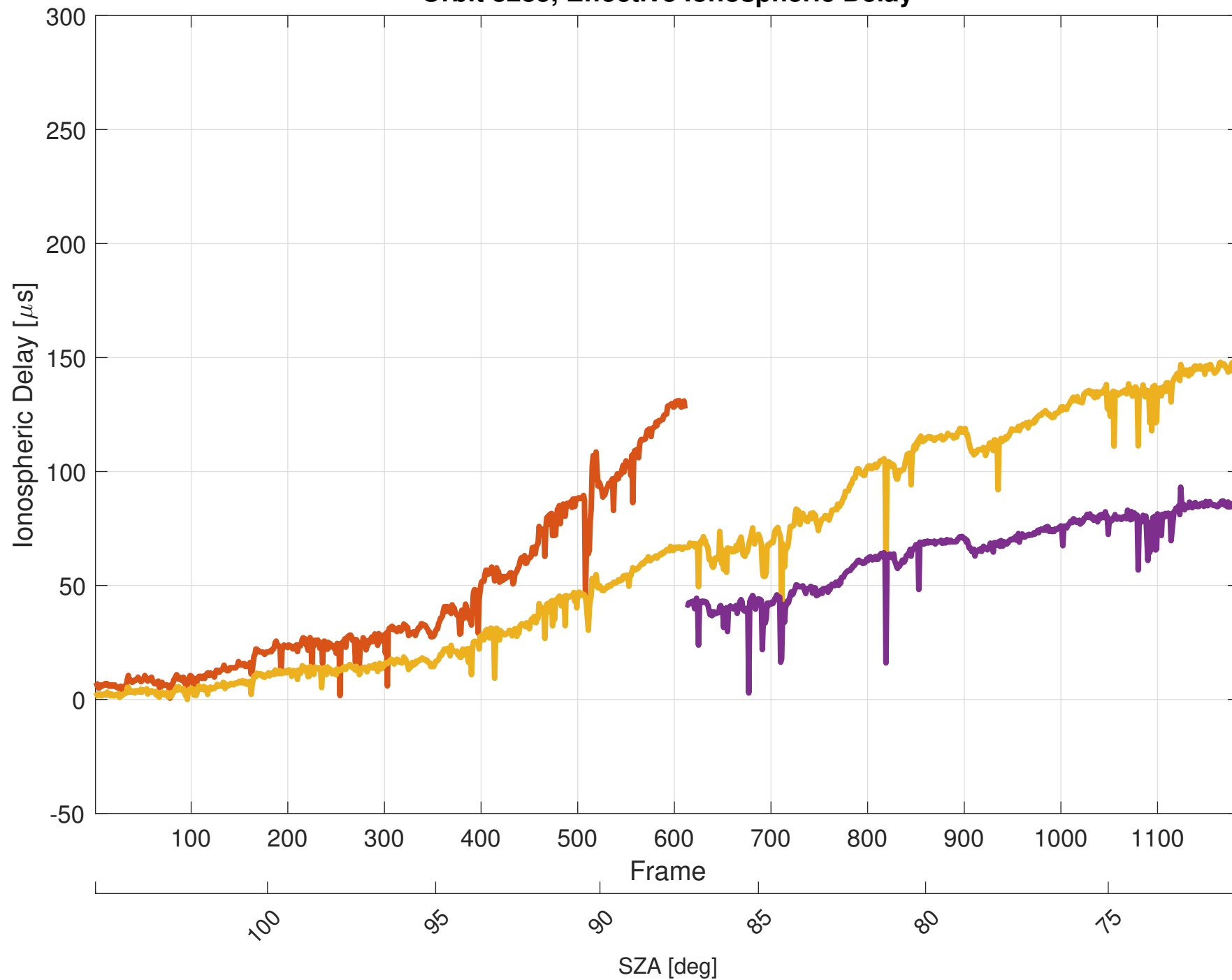
Orbit 8285, Effective Ionospheric Delay
