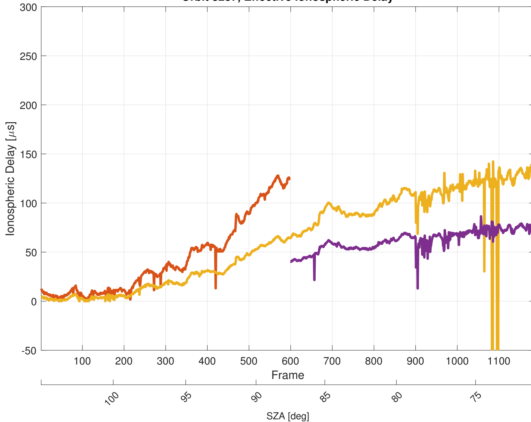
Orbit 8287, Effective Ionospheric Delay
