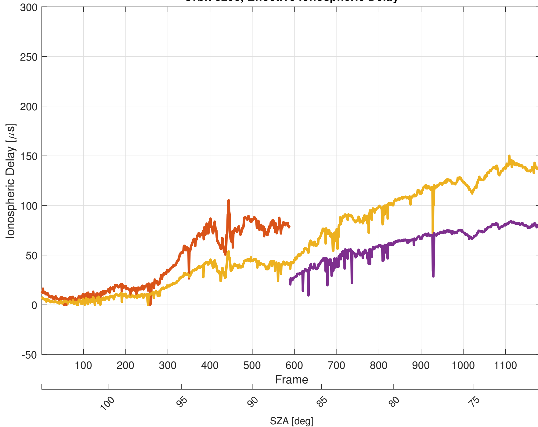
Orbit 8293, Effective Ionospheric Delay
