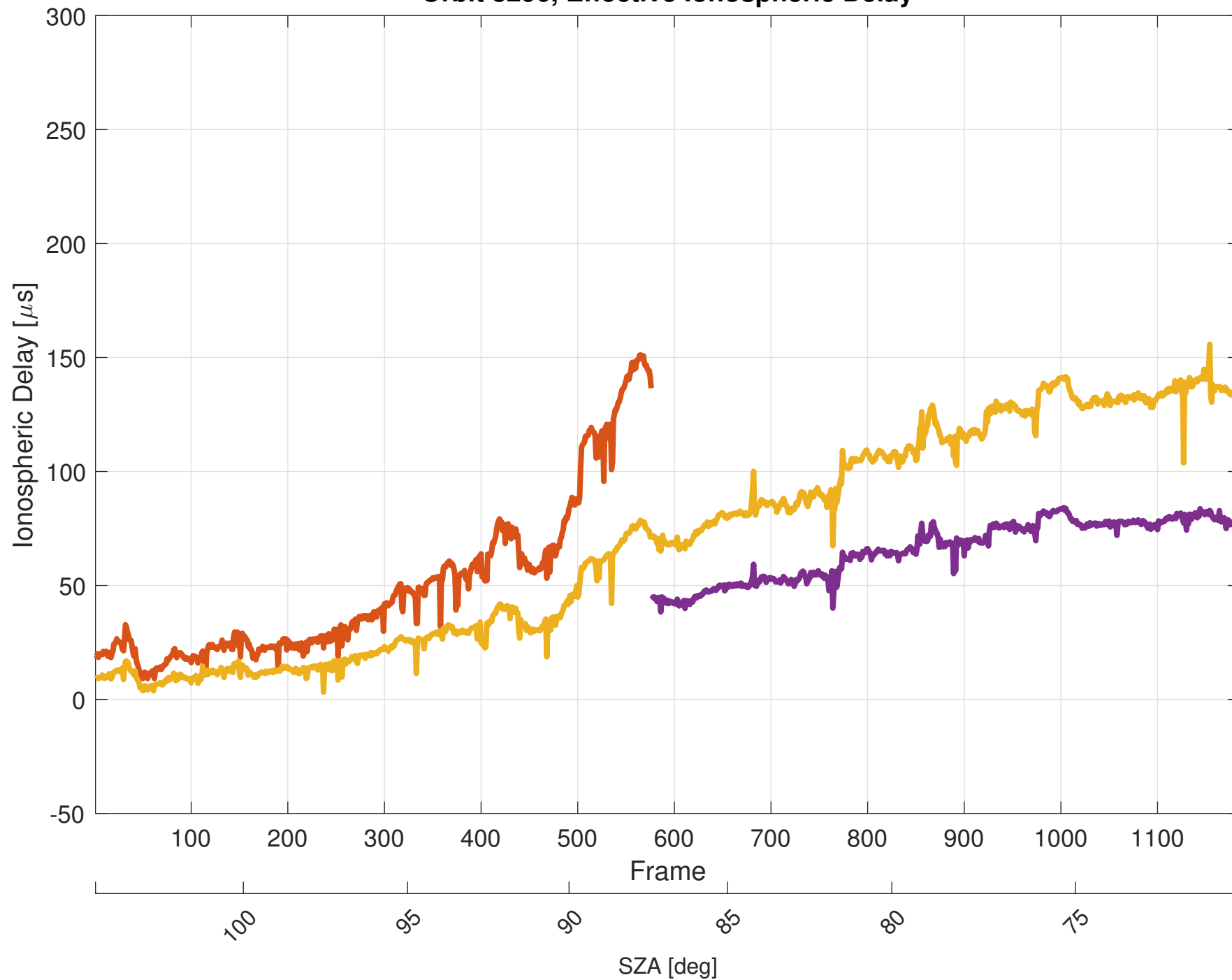
Orbit 8296, Effective Ionospheric Delay
